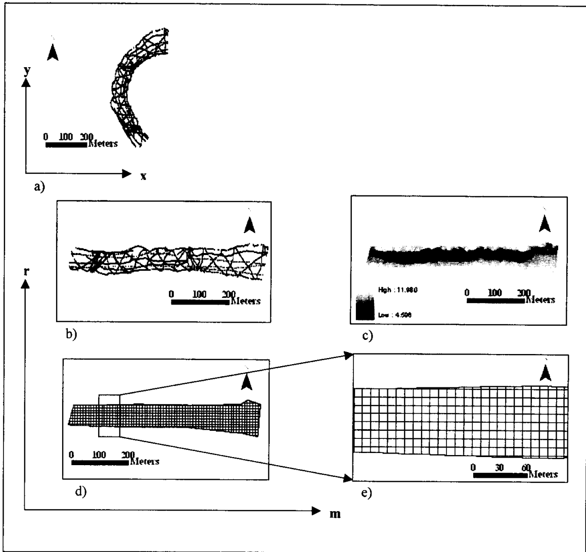
Figure 11. FishNet generation in (m,r) coordinates. (a) Small portion of the study reach in (x,y) coordinates; (b) Small portion transformed into (m,r) coordinates; (c) Grid generated for the small portion in (m,r) coordinates; (d) FishNet in (m,r) coordinates; (e) enlarged view of the FishNet, vertical lines are cross-sections and horizontal lines are profile lines.
