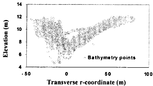
Figure10. Measurement points plotted against r axis in the (m,r) coordinate system.
