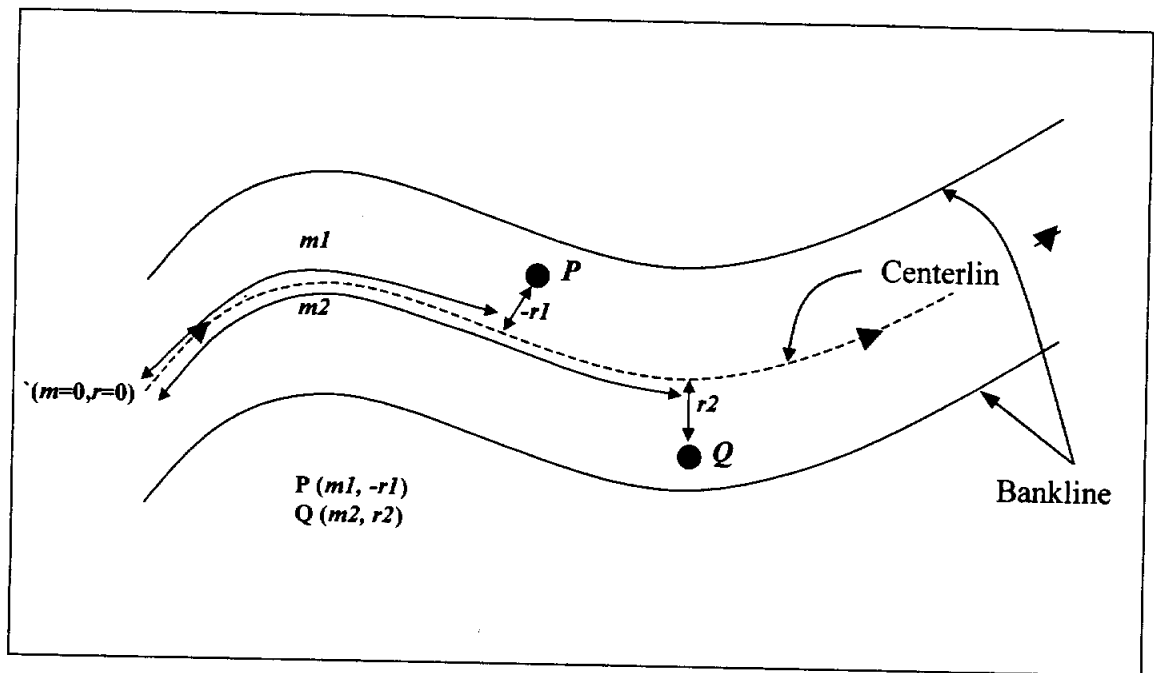
Figure 5. Hydraulic (m,r) coordinate system for a stream channel
