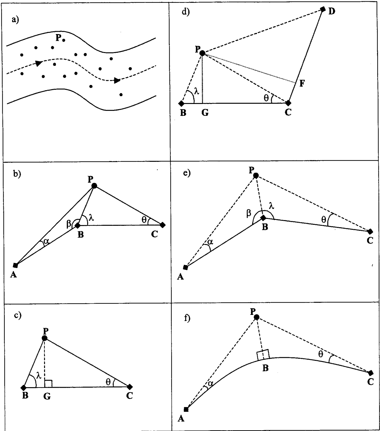
Figure 8. Geometric concepts for defining (m,r) coordinates for a bathymetry point P .
