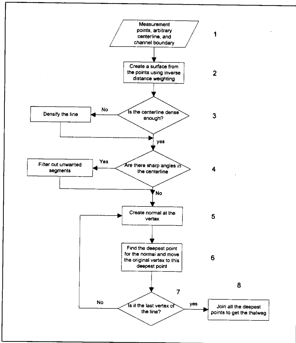
Figure 6. Flow chart for defining a Thalweg in GIS.
