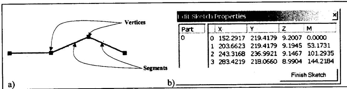
Figure 2. PolylineZM in ArcGIS. (a) A PolylineZM with its vertices and segments; (b) Properties of the each vertex of the PolylineZM.
