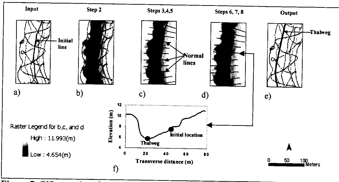
Figure 7. GIS procedure for the thalweg in GIS. (a) Input data; (b) Raster surface created using bathymetry points; (c) Normal lines created for the initial line at 15m interval; (d) initial line is moved to the deepest points along all the normals; (e) Final result with initial line changed to thalweg; (f) Vertical profile of a normal showing the location of initial line and the deepest point (thalweg).
