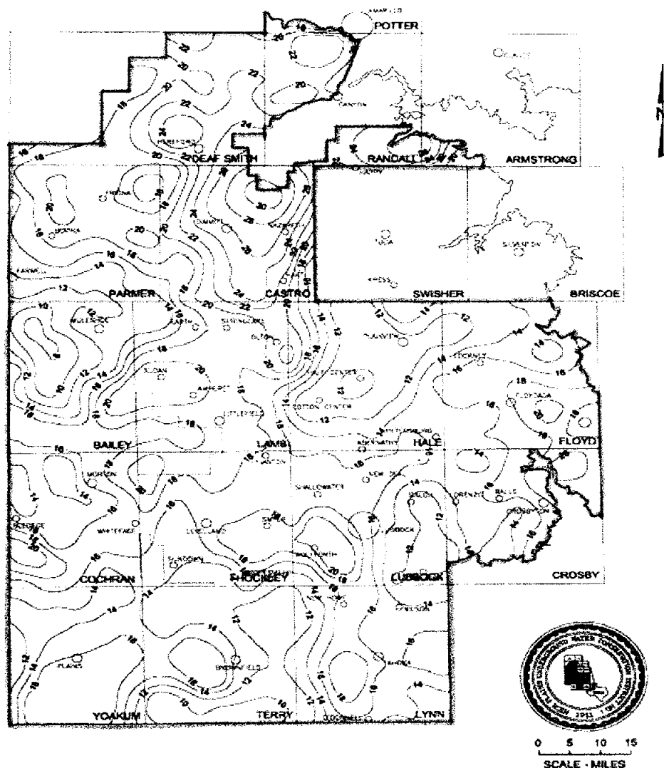
Figure 5. Isohyetal analysis (inches) in the seasonal (April through September) rainfall in 1999. The gauge maps were produced six months to a year prior to this study by personnel at the High Plains Underground Water Conservation District.
