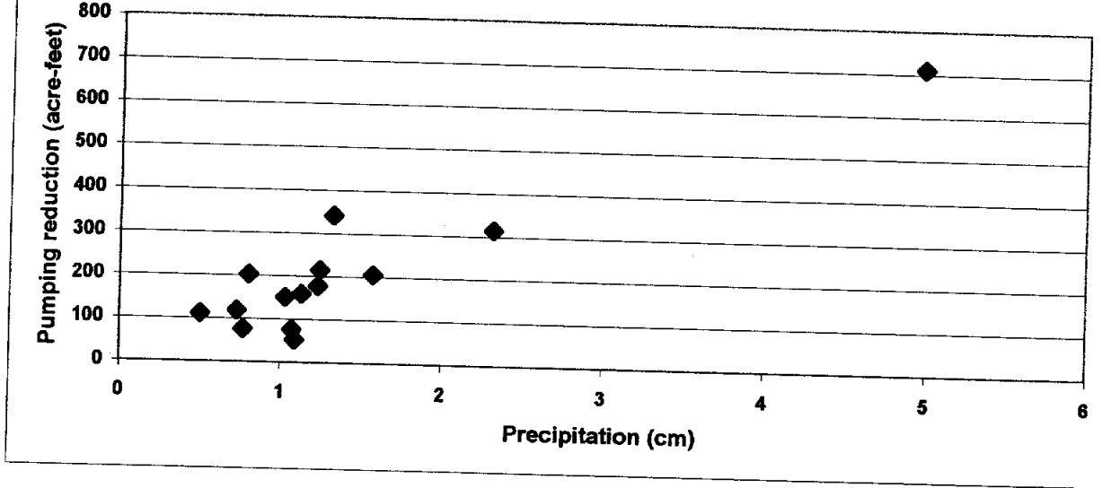
Figure 20: Effect of precipitation on pumping of the Edwards Aquifer by San Antonio (from data provided by Bexar Metropolitan Water District and San Antonio Water System)
