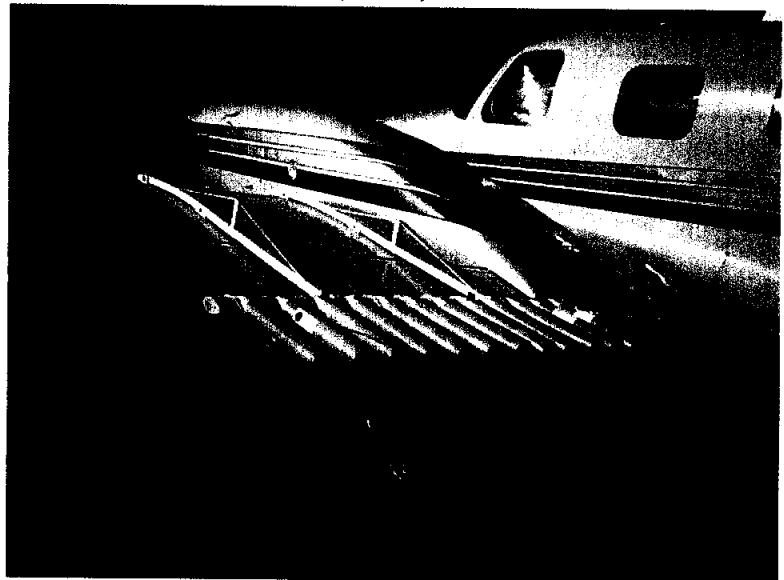
Figure 27. A wing rack of twelve 1 kg (1,000 g) yield hygroscopic cloud seeding flares. Each cloud turret is treated with a single flare, burned in updraft below cloud base.
