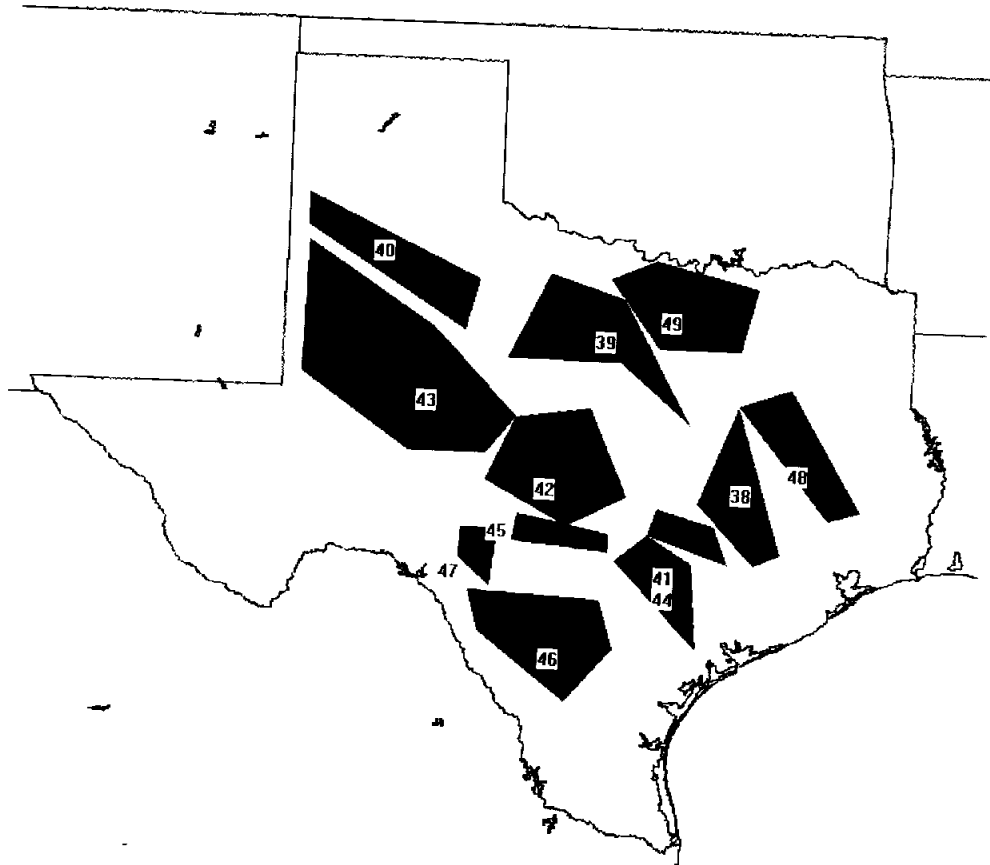
Figure 9. Map of 12 Texas drainage basins for which radar rainfall estimates were made. The key to the numbered areas is provided in Table 7.
