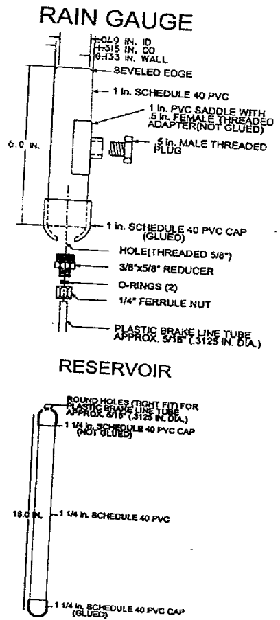
Figure 3. Design of the rain gauge system developed at the HPUWCD. a) the rain gauge assembly, b) the rain gauge, and c) the reservoir.
