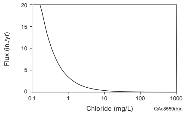
Figure 4. Sensitivity of drainage calculated using the chloride mass-balance approach to chloride concentrations, based on data from boreholes at a site in the Chihuahuan Desert, Texas, USA (Scanlon 2000).
