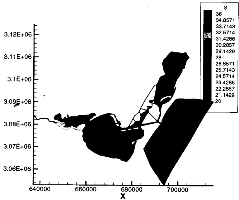
Figure 10: Salinity profile, day 28.9, layer 3
