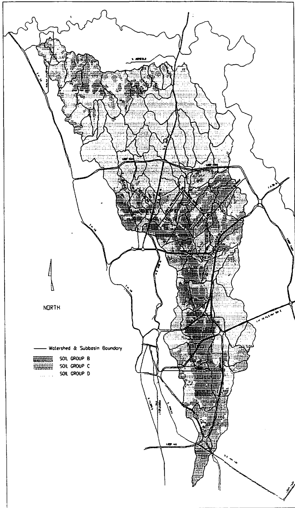
Figure 5 - "Soil Groups Within Salado Creek Watershed"
