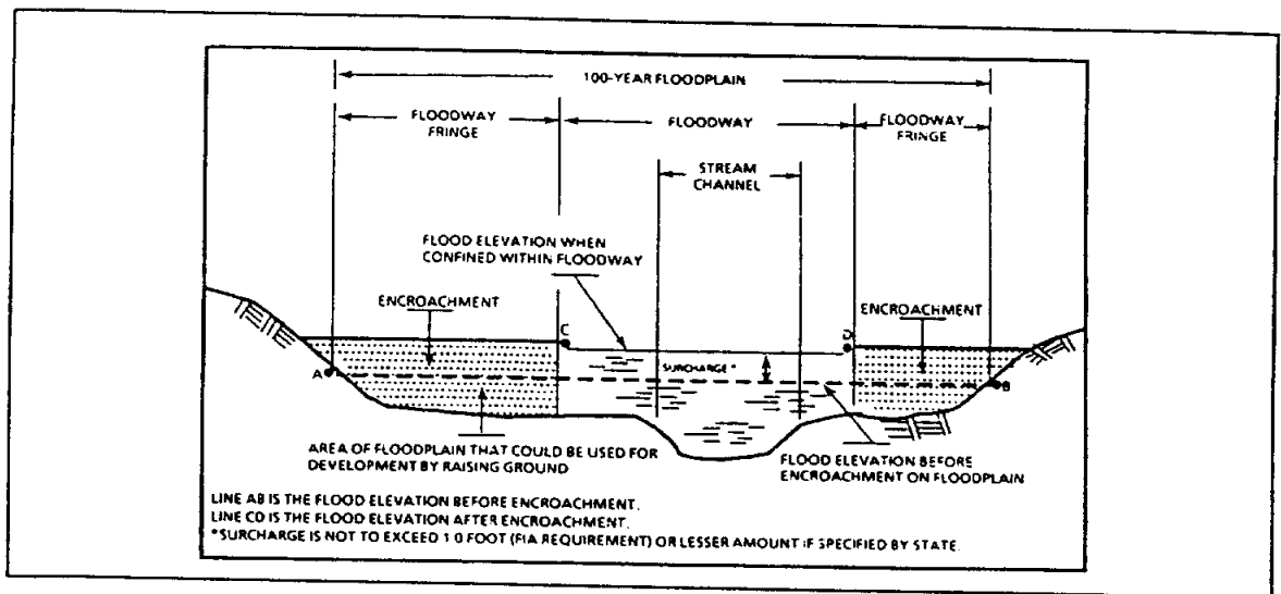
Figure 6. Floodway Schematic
