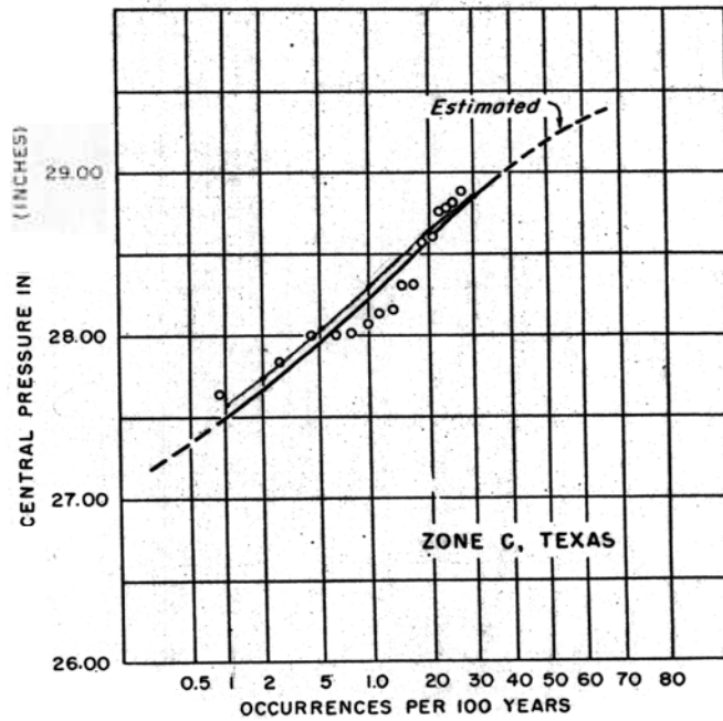
Figure 14. - Cumulative frequency of hurricane central pressure index (1900-1956 frequency per 100 years).
