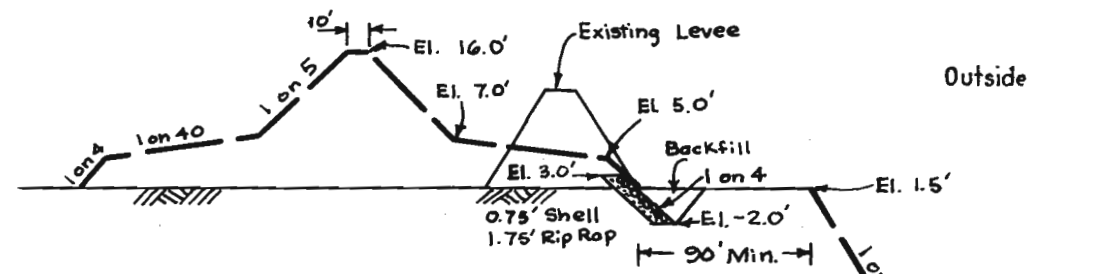
CITRUS BACK LEVEE (West of Paris Road)
