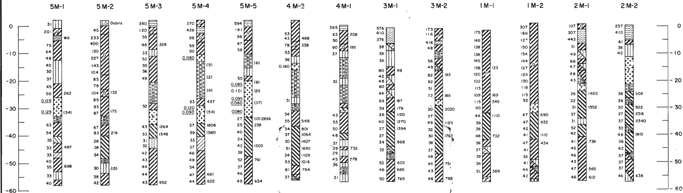
SOIL BORING LOGS
