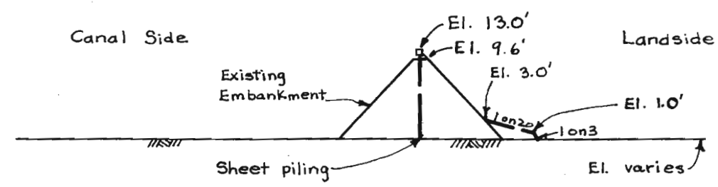
INNER HARBOR NAVIGATION CANAL Sheet Piling Enlargement
