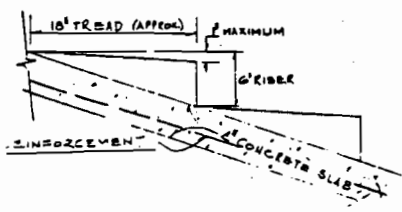
DETAIL OF STEP CONSTRUCTION
