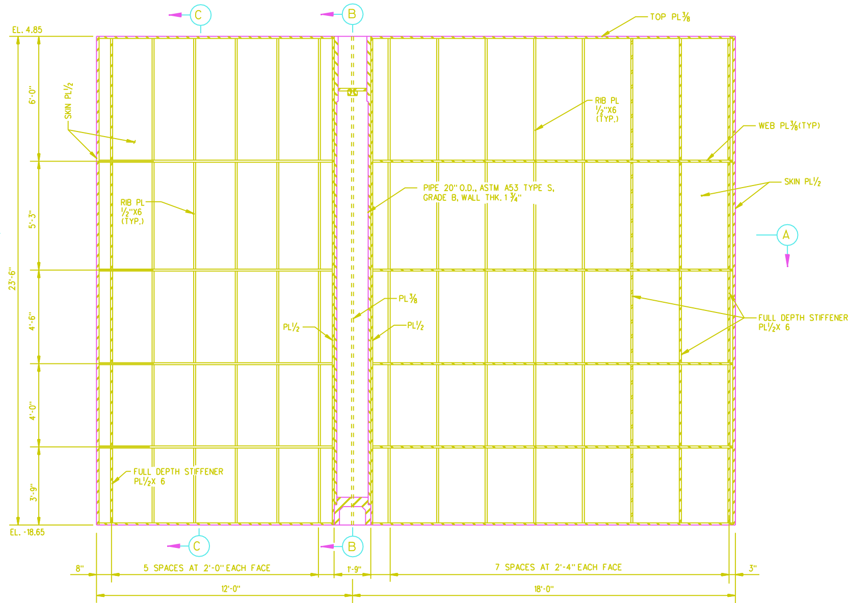
SECTION ALONG CENTER LINE OF GATE
