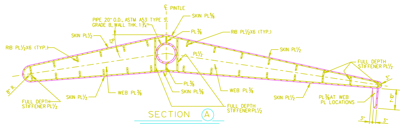
SECTION ALONG CENTER LINE OF GATE
