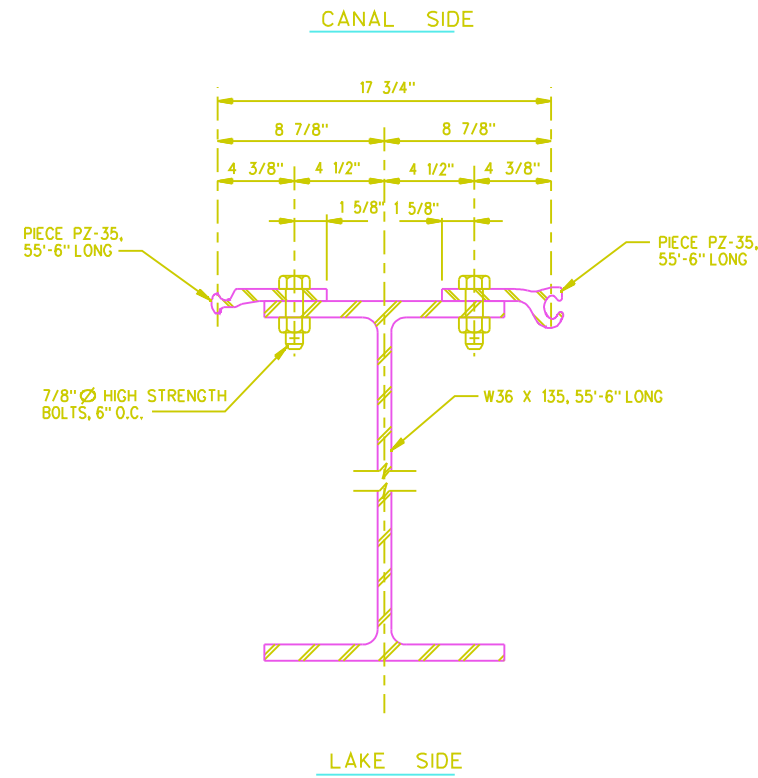
SPECIAL W36 X 135 PILE DETAIL SCALE: 3" = 1'-0"
