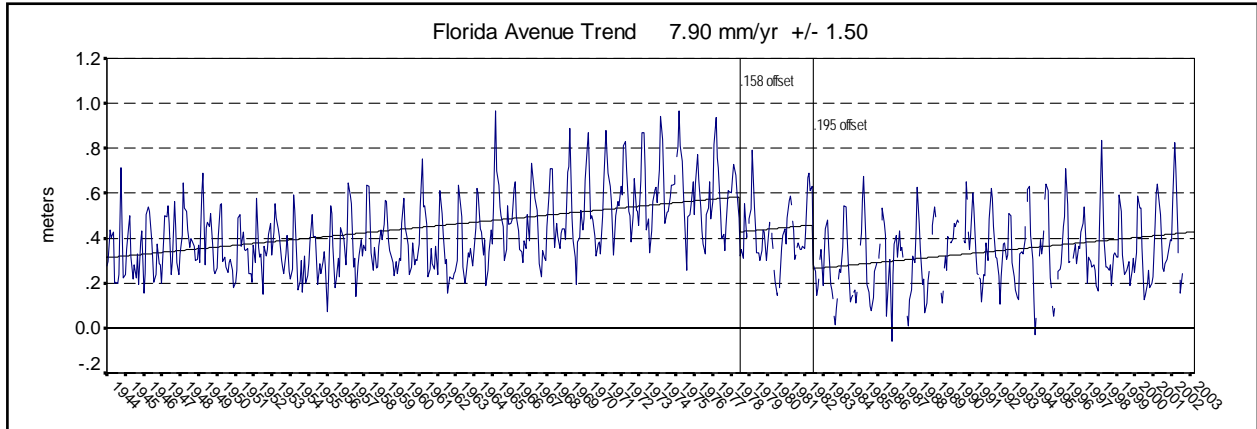
Figure 52. Apparent sea level rise at Corps IHNC Florida Ave. gage 1944 to 2003 (Source: IPET MVN and NOAA CO-OPS).
