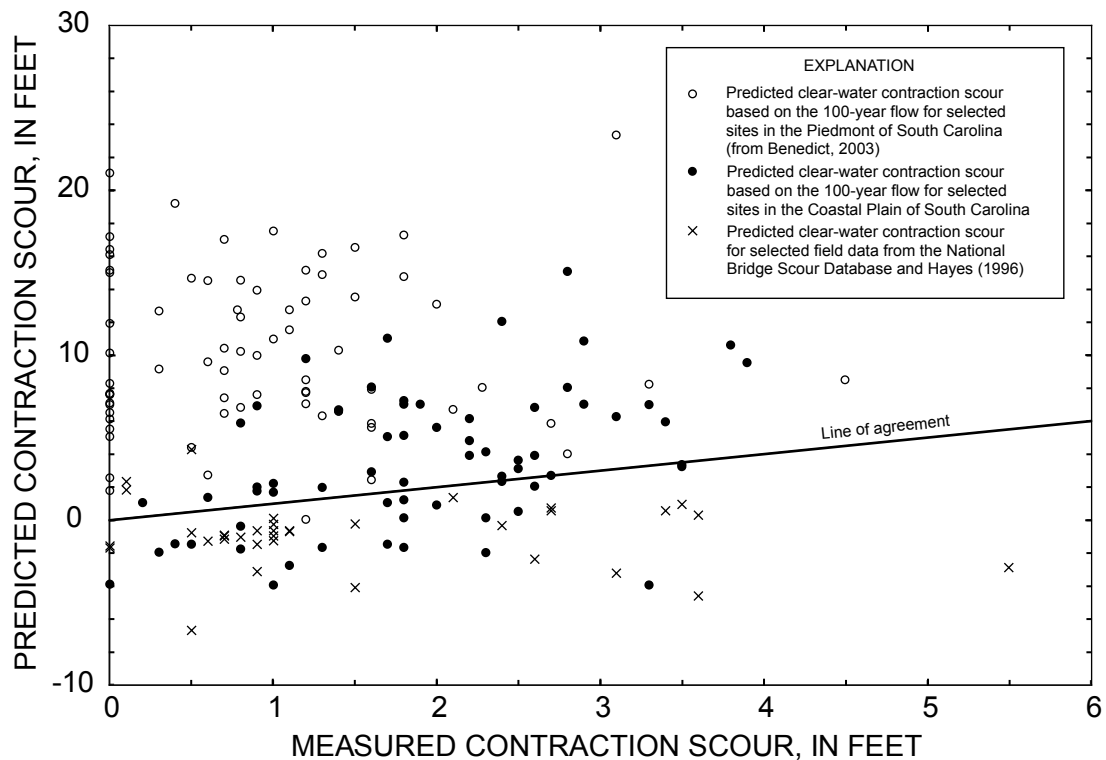
Figure 67. Relation of measured clear-water contraction-scour depth to predicted contraction-scour depth for selected sites in the Coastal Plain and Piedmont Physiographic Provinces of South Carolina, and from the National Bridge Scour Database and Hayes (1996). (Predicted clear-water contraction scour was calculated with the HEC-18 equation (Richardson and Davis, 2001).)
