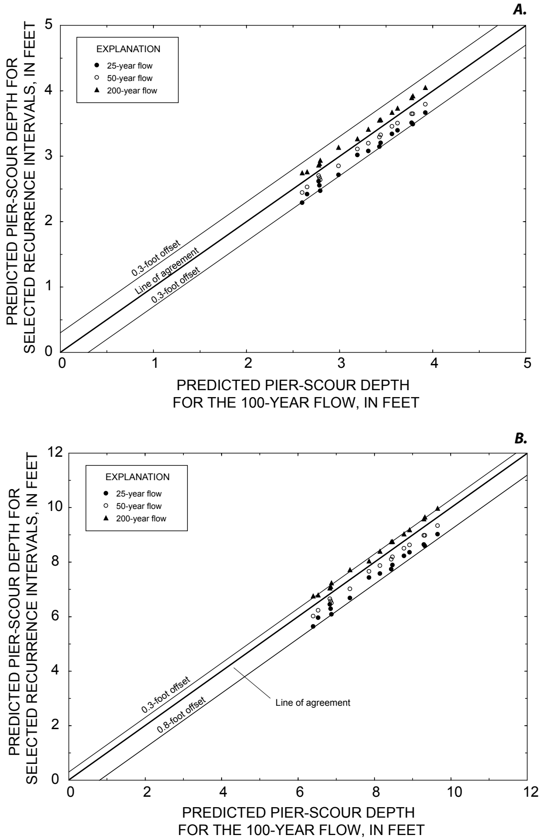
Figure 25. Relation of theoretical pier scour for the 25-, 50-, and 200-year flows with respect to the 100-year flow at selected bridges in South Carolina for (A) a pier width of 1.5 feet and (B) a pier width of 6 feet.
