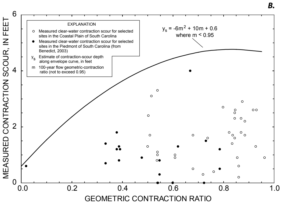
Figure 69. Relation of measured clear-water contraction-scour depths to the geometric contraction ratio at selected sites in the Coastal Plain and Piedmont Physiographic Provinces of South Carolina for (A) the 100-year flow and (B) the maximum historic flows.
