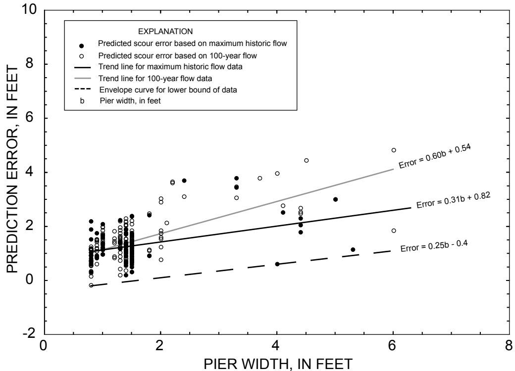
Figure 55. Relation of pier width to prediction error using hydraulic variables for the 100-year flow and known maximum historic flows at selected sites in South Carolina. (Predicted pier scour was calculated with the HEC-18 pier-scour equation (Richardson and Davis, 2001) with all correction coefficients set to 1.)
