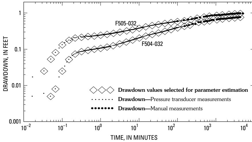
Figure D. Drawdown data for piezometers F505-032 and F504-032.
