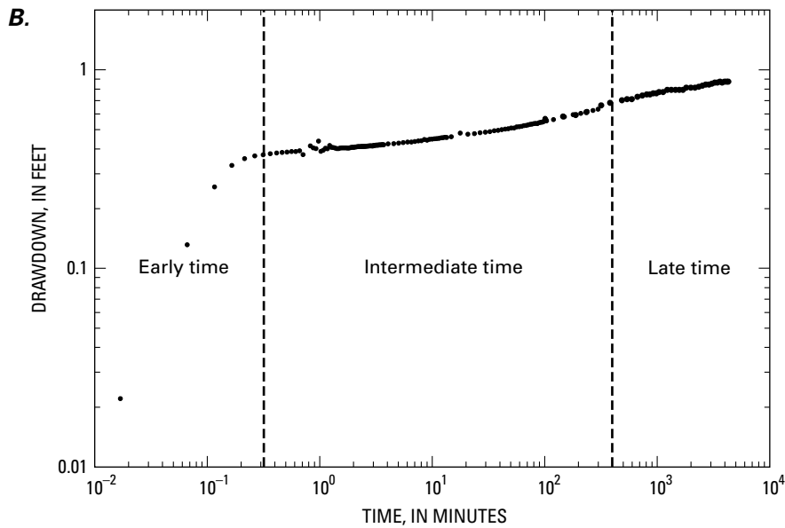
Figure 1. A. Schematic diagram of a pumping well and observation piezometer in an idealized, anisotropic unconfined aquifer with a hypothetical moisture distribution indicated for the unsaturated zone. B. A typical double-logarithmic plot of drawdown in an observation piezometer versus time that defines the approximate ranges of early-, intermediate-, and late-time.
