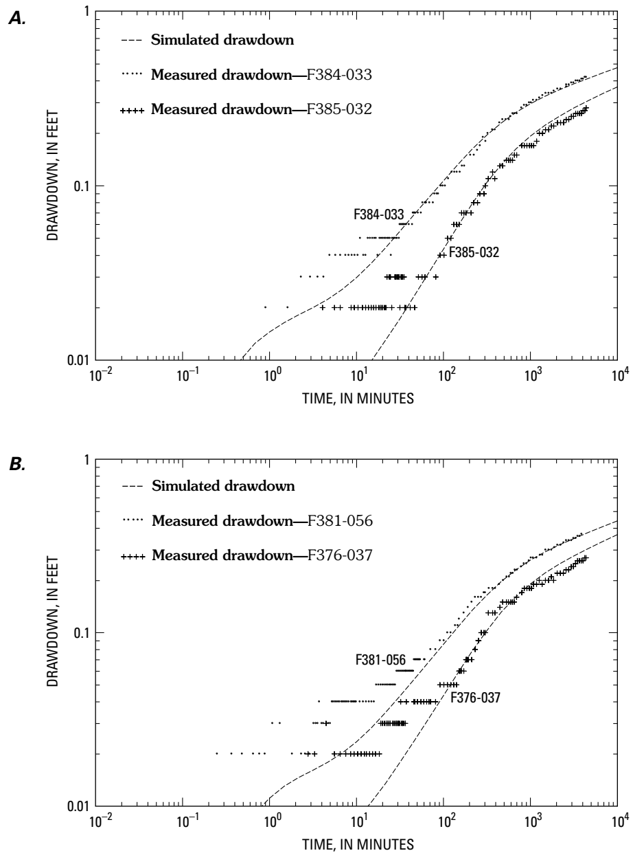
Figure 19. Measured drawdowns compared with drawdowns simulated under the assumption of gradual release of water from the unsaturated zone, ( A ) piezometers F384-033 and F385-032, and ( B ) piezometers F381-056 and F376-037.
