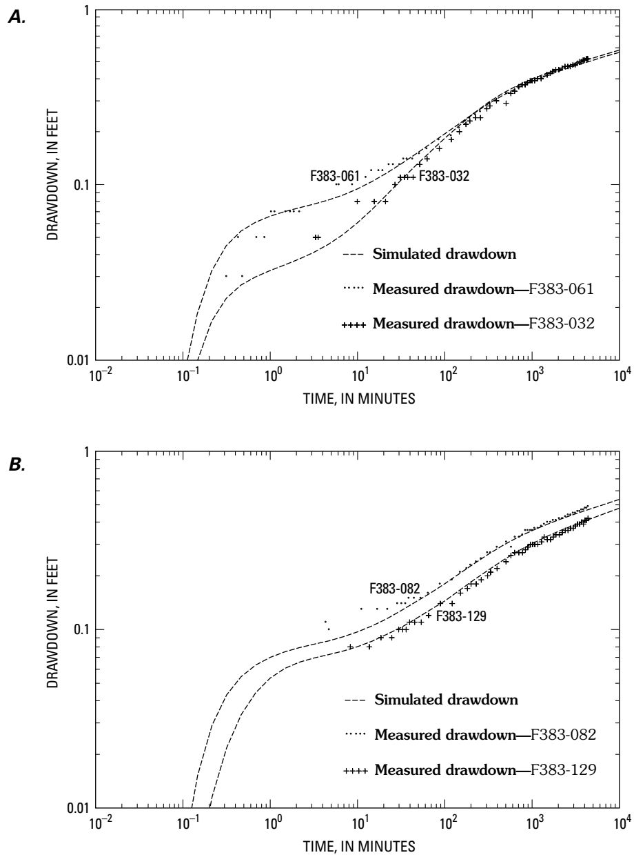
Figure 18. Measured drawdowns compared with drawdowns simulated under the assumption of gradual release of water from the unsaturated zone, (A) piezometers F383-061 and F383-032, and (B) piezometers F383-082 and F383-129.
