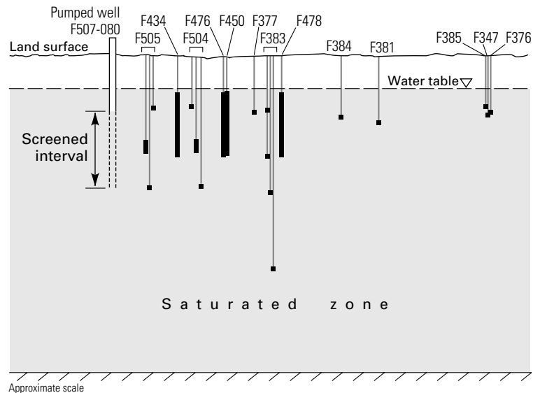
EXPLANATION F384 — Well identification number — Observation well — Screened interval(s) of observation wells and piezometers Figure 4. Vertical cross section of the aquifer at the study site showing the lengths and positions of the piezometers and observation wells.
