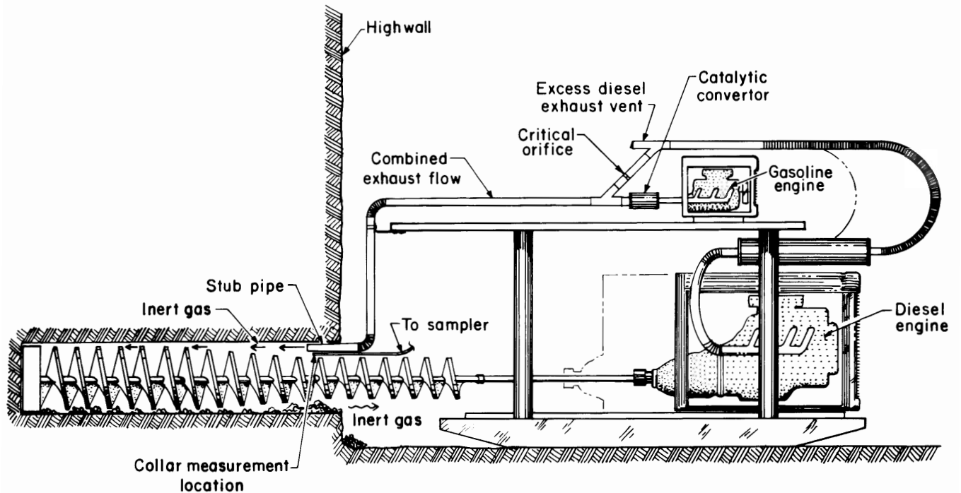
Figure 3.—Schematic of inert gas system as tested.
