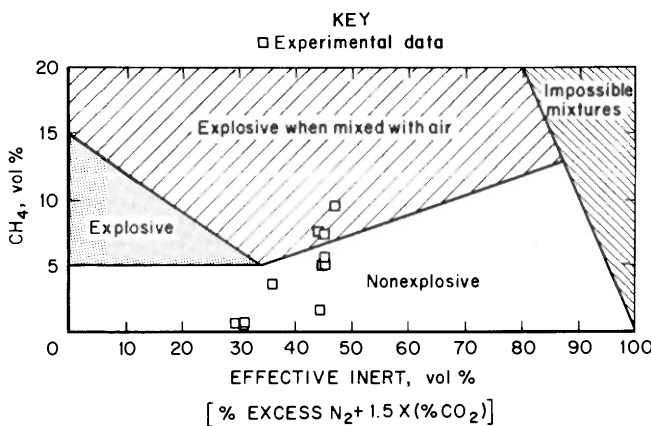
Figure 6.—Explosibility diagram for March data with observed gas concentrations plotted for all holes.
