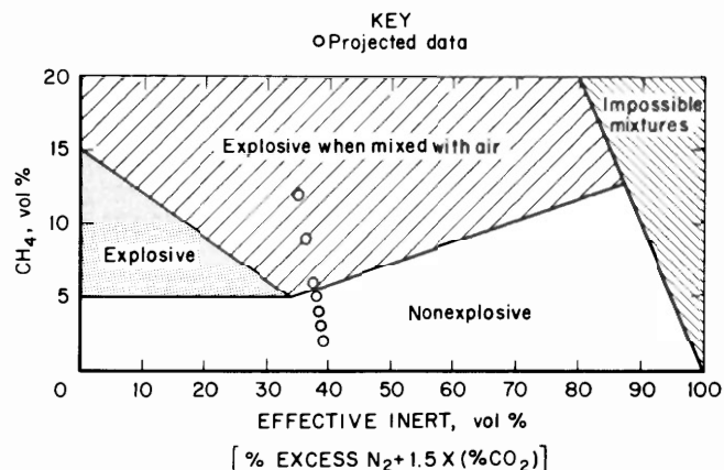
Figure 5.—Explosibility diagram for January. Gas data projected as if various levels of methane were encountered.
