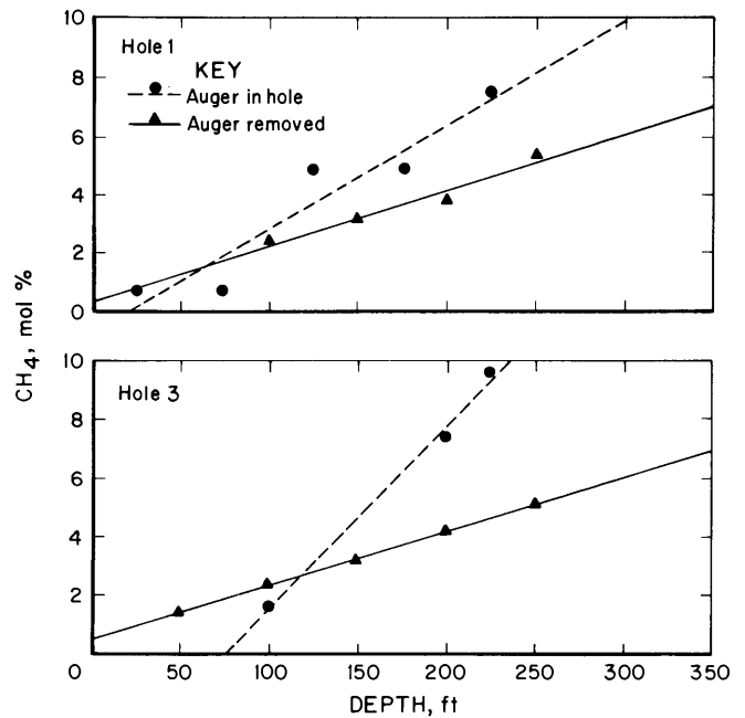
Figure 7.—Profiles of methane concentrations in holes 1 and 3 at maximum hole depth with augers in place, and immediately after auger removal.
