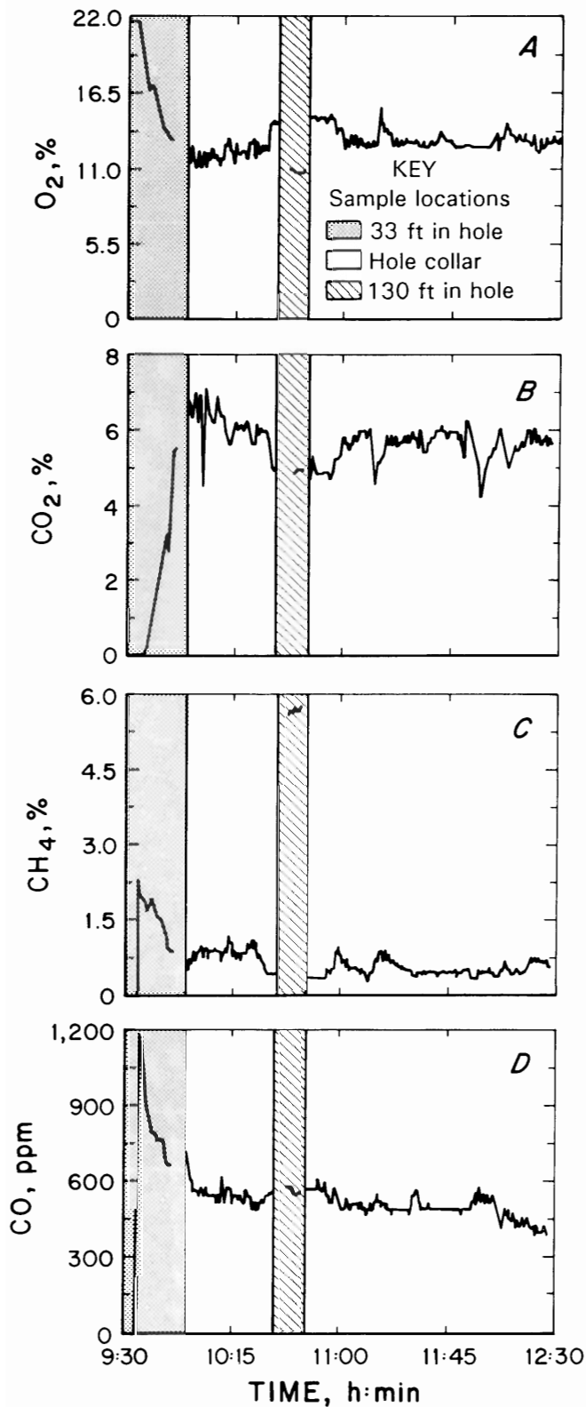
Figure 8.—Corrected infrared gas concentrations at the collar sample location for hole 3. Note data at 10:44 and initial inerting of hole were not collar samples.
