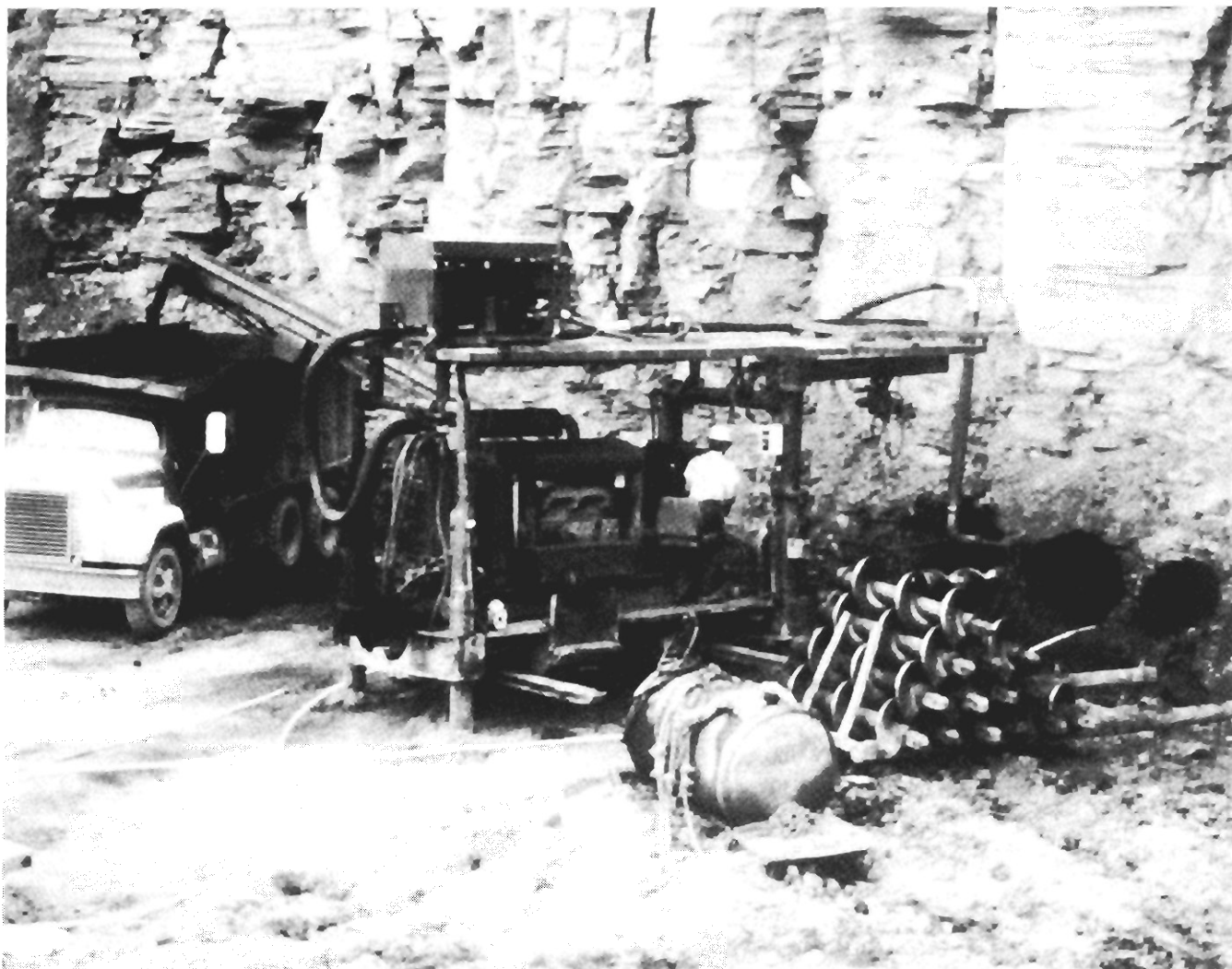
Figure 4.—Overview of highwall mining operation as tested.
