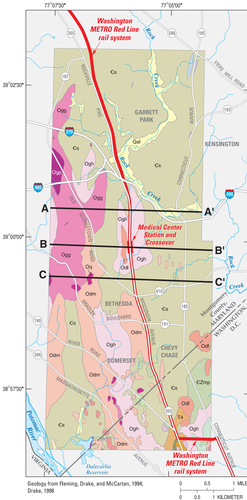
Figure 3. Regional geology near the Medical Center Station and Crossover, Montgomery County, Maryland, and locations of geologic cross sections A-A', B-B', and C-C'.
