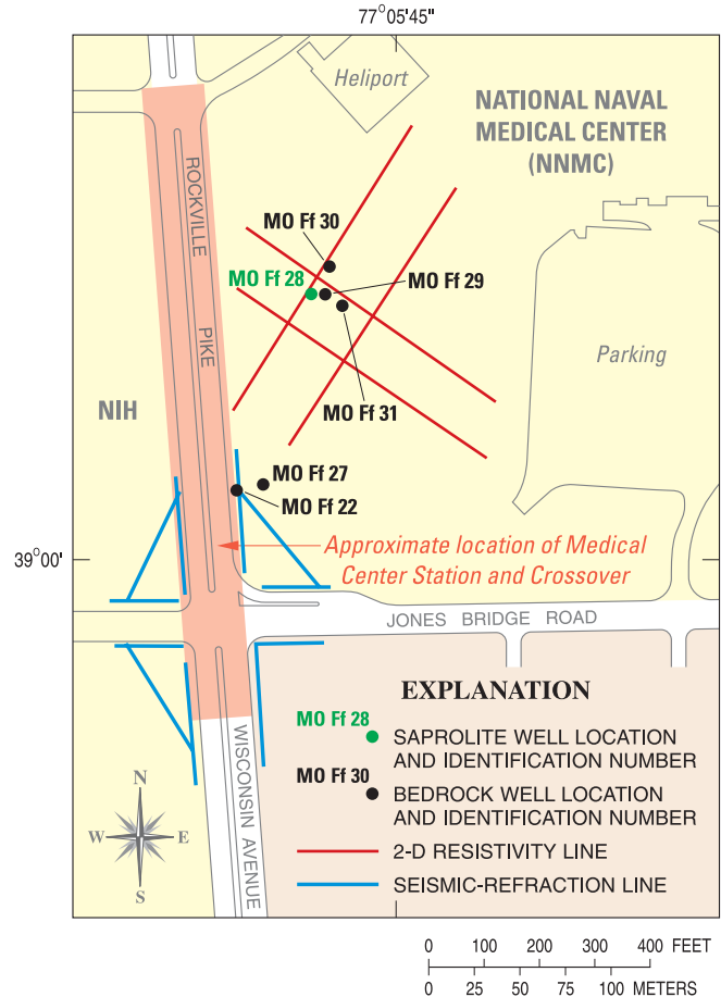
Figure 9. Location of National Naval Medical Center well field, seismic-refraction lines, and 2-D resistivity lines.
