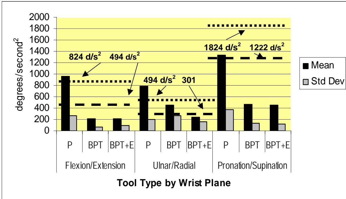
Figure 9 Measured Wrist Acceleration during Rebar Tying
