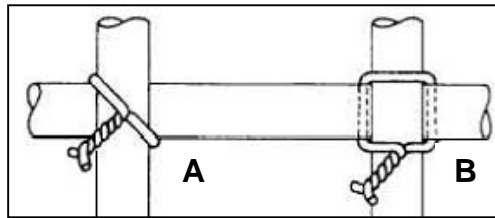
Figure 2 Ties used to secure rebar together
