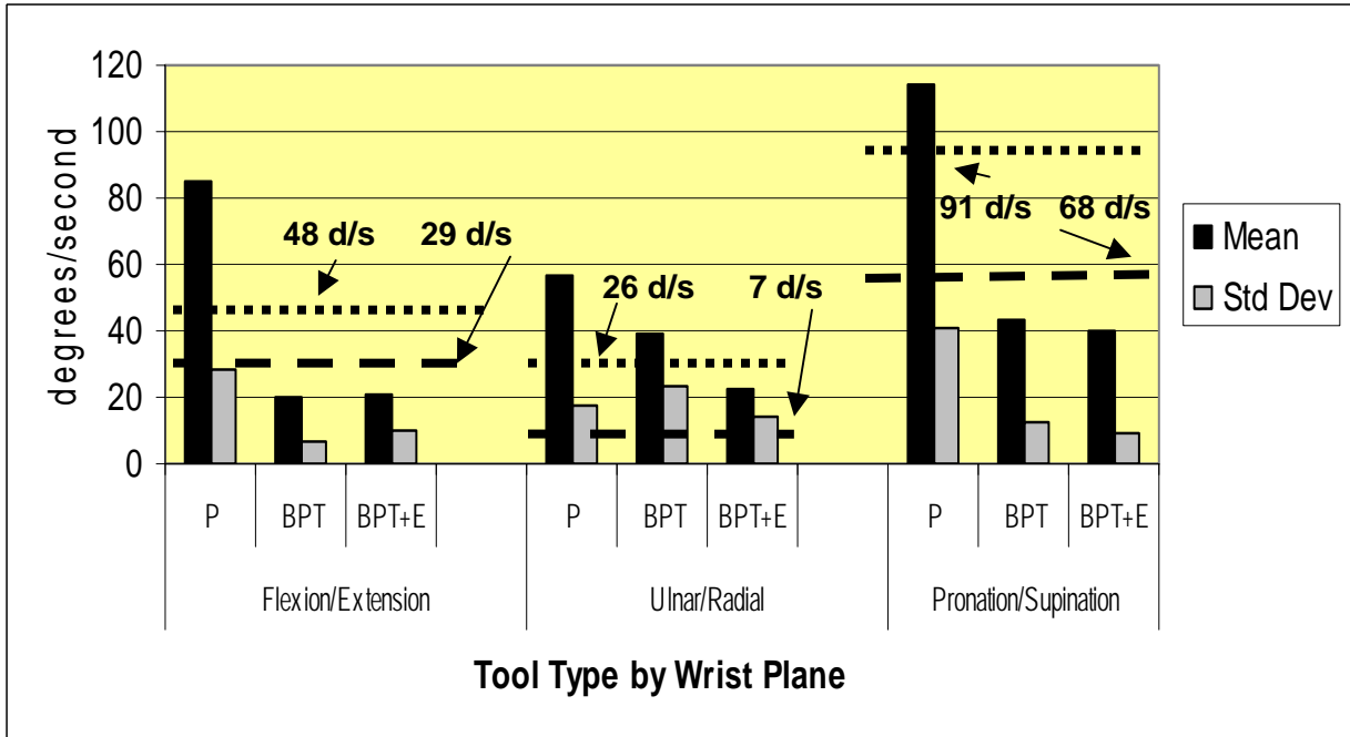
Figure 8 Measured Wrist Velocity during Rebar Tying
