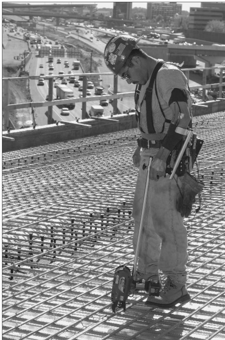
Figure 6 Rebar tying using MAX-USA RB392 power rebar tier with adjustable extension handle
