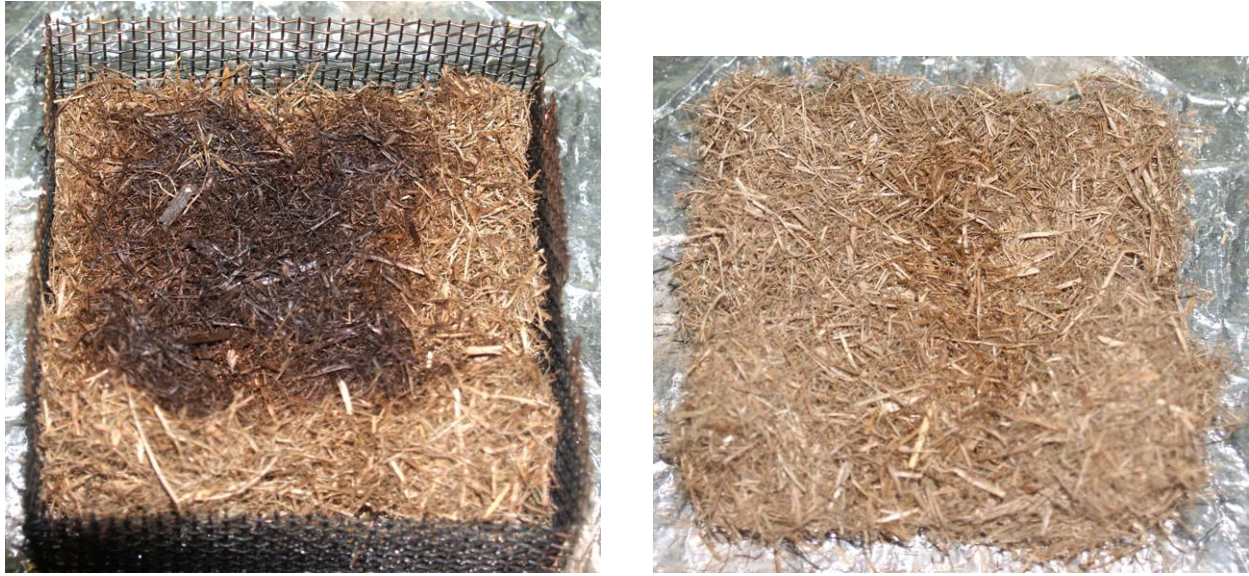
Figure 59. Bottom (left) and top (right) views of a fine Florida grass fuel bed are shown after the fuel was removed from the heated plate held at 290 °C with a low wind applied. Glowing combustion was not observed.
