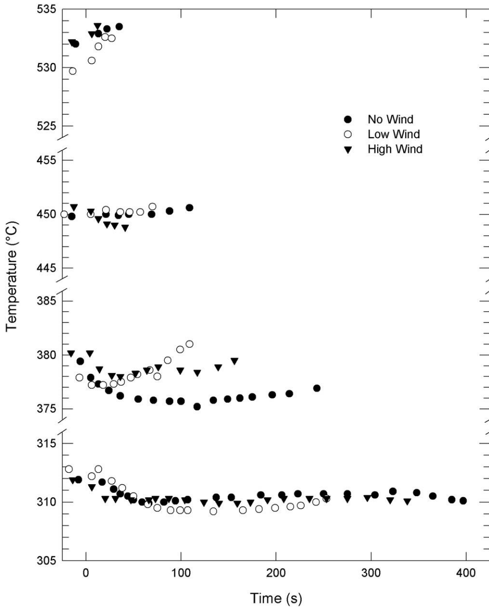
Figure 9. Temperatures recorded during experiments in which cellulose fuels were placed on a heated plate are plotted as a function of time. Zero time is defined as the time when the fuel was exposed to the surface.
