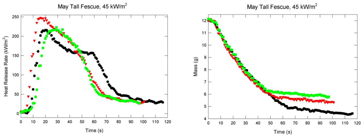
Figure 39. Heat release rates and sample masses are plotted as a function of time for three experiments in which a 45 \text{ kW/m}^2 heat flux was applied to May tall fescue.
