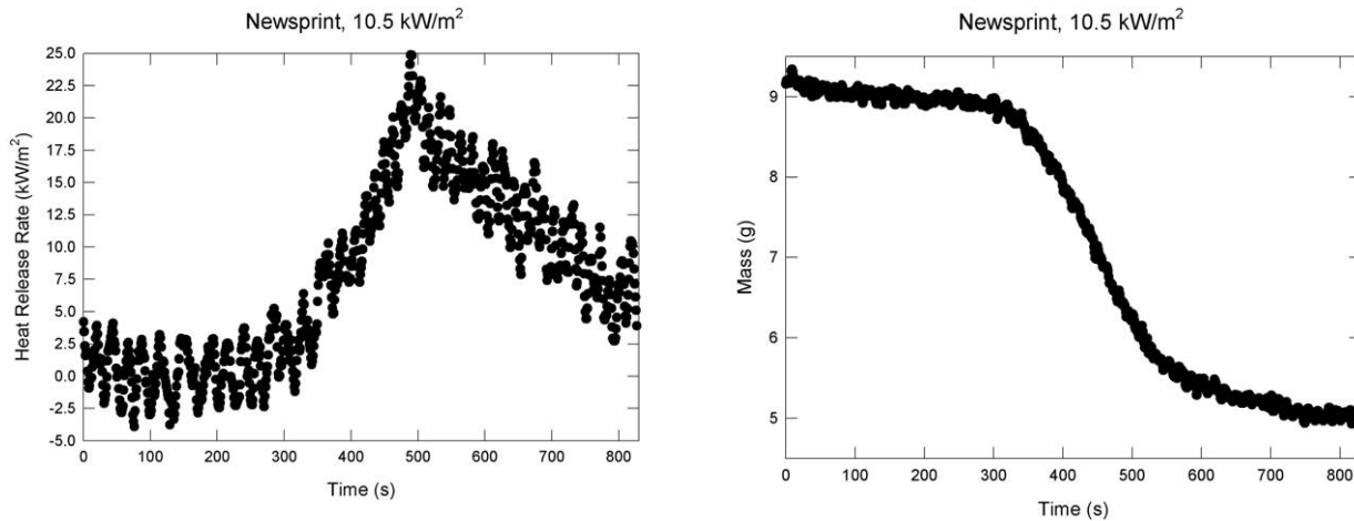
Figure 31. Heat release rates and sample masses are plotted as a function of time for an experiment in which a 10.5 kW/m 2 heat flux was applied to shredded newsprint.
