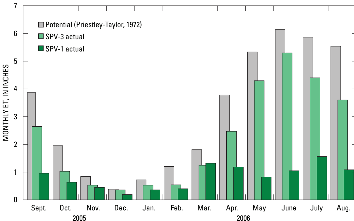
Figure 14. Monthly potential evapotranspiration (PET) and evapotranspiration (ET) measured at grassland/meadowland ET site SPV-3, and ET measured at sparse desert shrubland ET site SPV-1, Basin and Range carbonate-rock aquifer system study area, Nevada and Utah September 1, 2005, to August 31, 2006.
