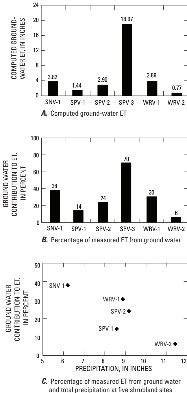
Figure 18. Annual ground-water contribution to measured evapotranspiration (ET) in Basin and Range carbonate-rock aquifer system study area, Nevada and Utah, September 1, 2005, to August 31, 2006.
