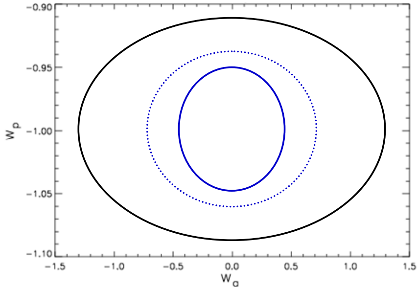
Illustration of the potential improvement in the DETF figure of merit arising from Stage III projects in the w_\alpha - w_p plane. The DETF figure of merit is the reciprocal of the area enclosed by the contours. The outer contour corresponds to Stage II, and the inner contours correspond to pessimistic and optimistic ALL-photo. All contours are 95% C.L.
