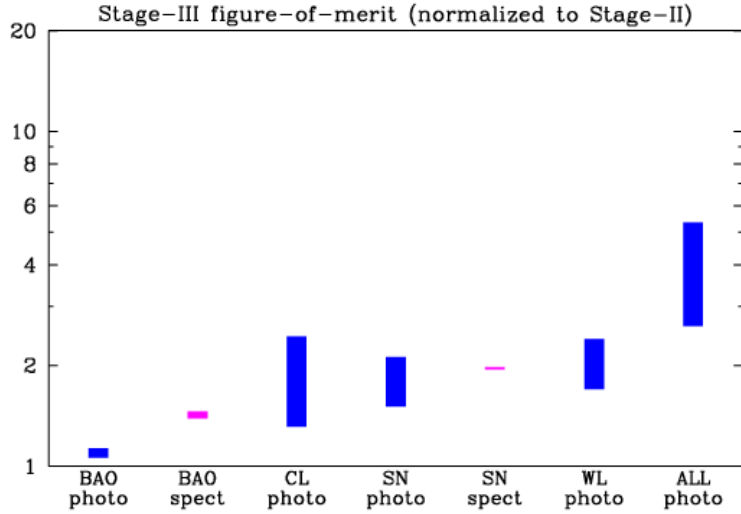
Illustration of the potential improvement in the DETF figure of merit arising from Stage III projects. The improvement is given for the different techniques individually, along with various combinations of techniques. In the figure ‘photo’ and ‘spect’ refers to photometric and spectroscopic surveys, respectively. Each bar extends from the expectation with pessimistic systematics up to the expectation with optimistic systematics. “ALL photo” combines photometric survey results from BAO, CL, SN, and WL.
