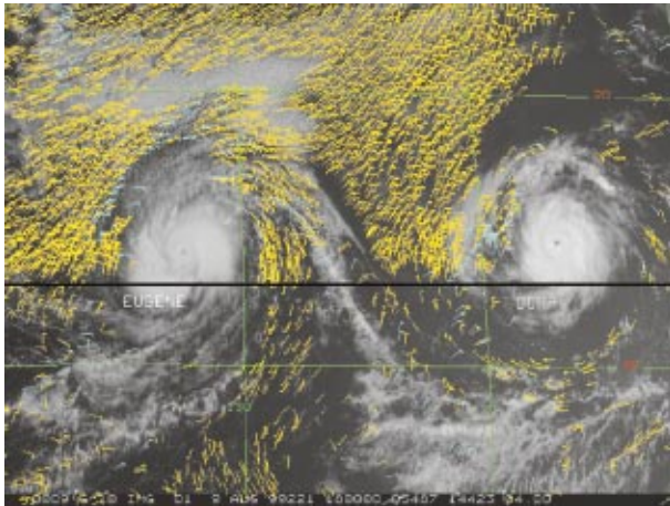
This image shows low-level visible cloud-drift winds around hurricanes Eugene and Dora. Three 15-minute sectors (above the horizontal black line) and three 30-minute sectors (below the black line) were used to derive the visible winds from Imager data. Note the significant improvement in detail of the wind field from data that was obtained in 15-minute intervals in the top half of the image. The straight end of each wind barb points in the direction that the wind is blowing.
