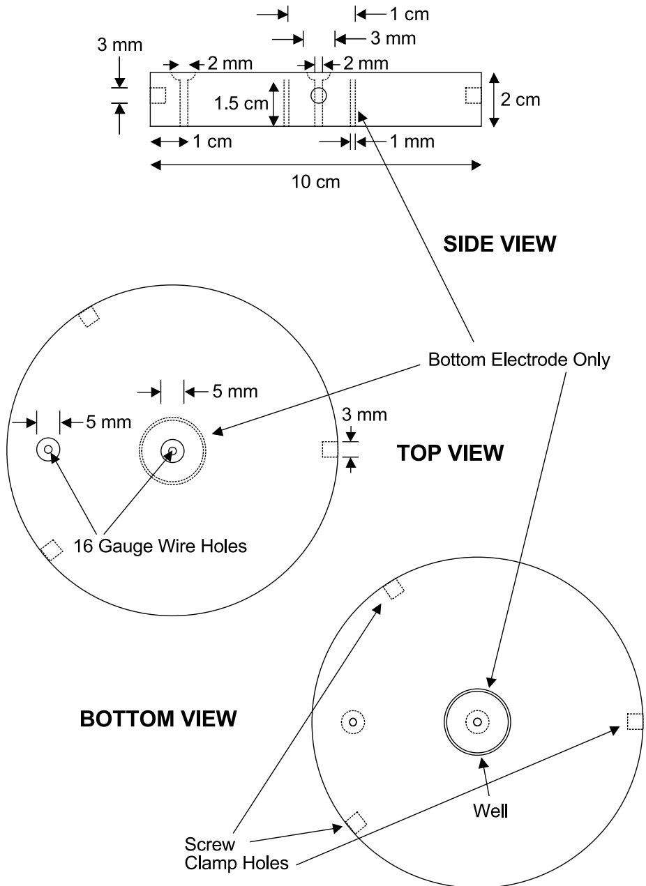
Figure 1. Fused quartz blank electrode construction. Note that the drawing is not to scale; the supplied measurements should be used. (The diameter of the blank is 10 cm as specified in the text.)
