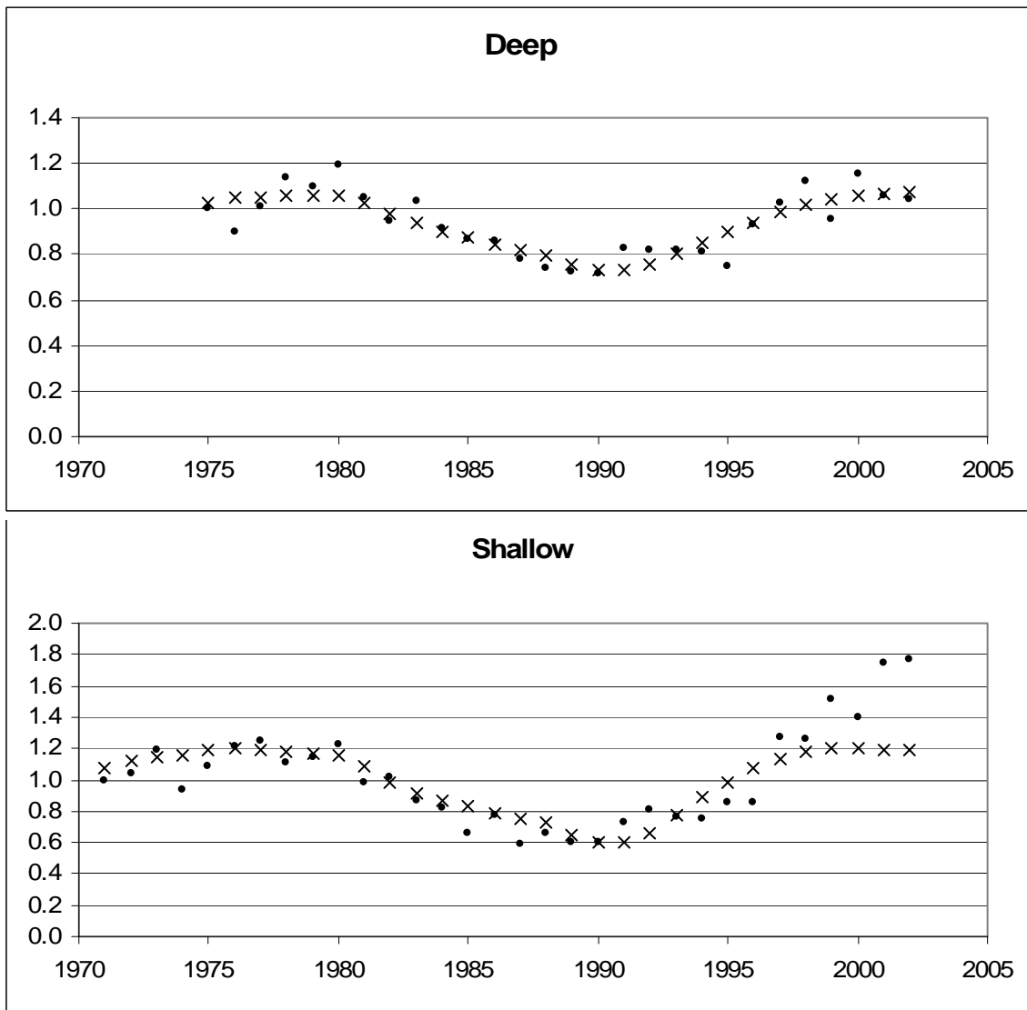
Figure 11.--Fit of the BSP model predicted CPUE ( \times ) for deep (1975–2002) and shallow (1971–2002) sets to the observed deep and shallow CPUE indices ( \bullet ).
