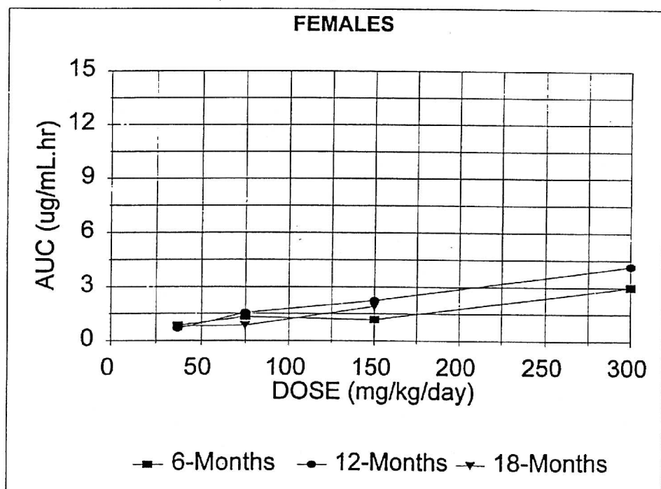
FIGURE I4 Plots of AUC Versus Dose for Methyleugenol in Rats at the 6-, 12-, and 18-Month Interim Evaluations in the 2-Year Gavage Study of Methyleugenol
