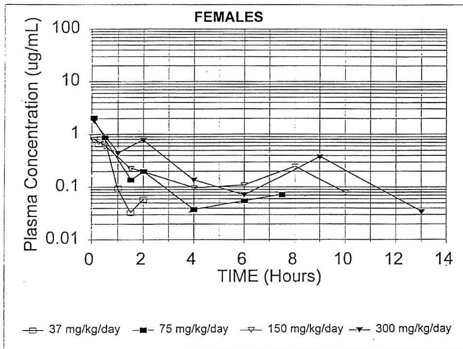
FIGURE I2 Plasma Concentrations of Methyleugenol in Rats at the 12-Month Interim Evaluation in the 2-Year Gavage Study of Methyleugenol
