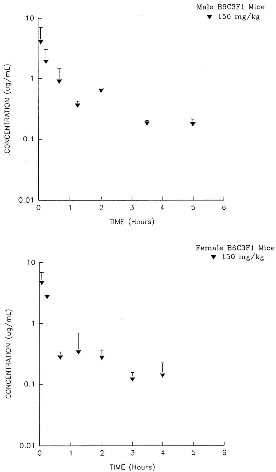
FIGURE I8 Plasma Concentrations of Methyleugenol in Mice Administered 150 mg/kg Methyleugenol at the 12-Month Interim Evaluation in the 2-Year Gavage Study of Methyleugenol
