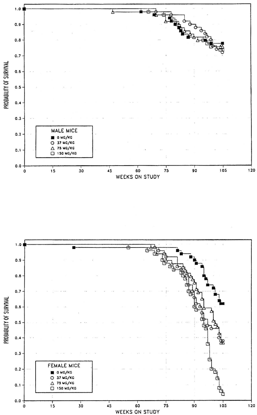
FIGURE 3 Kaplan-Meier Survival Curves for Male and Female Mice Administered Methyleugenol by Gavage for 2 Years
