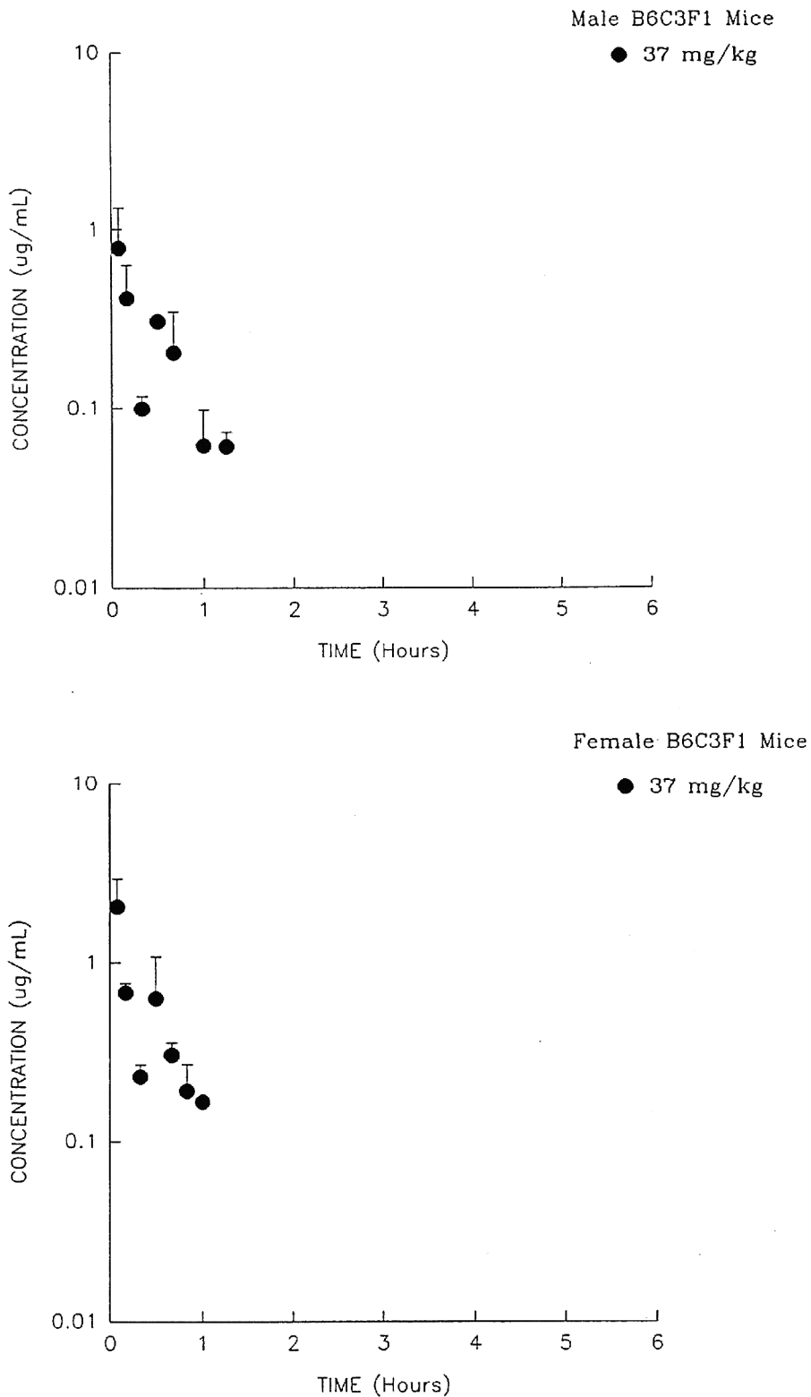
FIGURE I6 Plasma Concentrations of Methyleugenol in Mice Administered 37 mg/kg Methyleugenol at the 12-Month Interim Evaluation in the 2-Year Gavage Study of Methyleugenol
