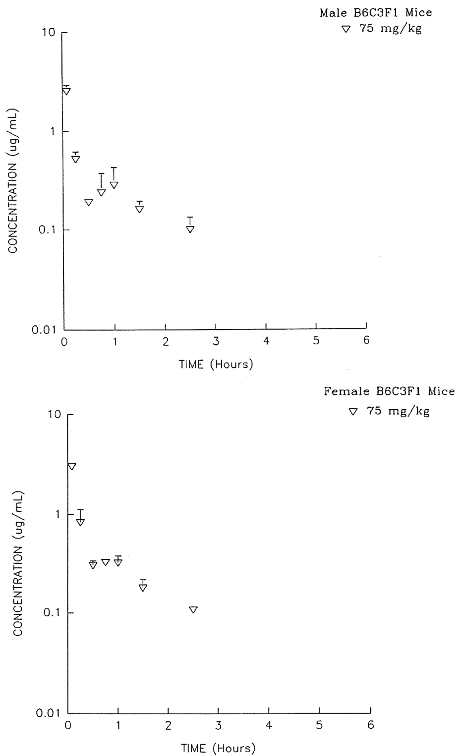
FIGURE I7 Plasma Concentrations of Methyleugenol in Mice Administered 75 mg/kg Methyleugenol at the 12-Month Interim Evaluation in the 2-Year Gavage Study of Methyleugenol
