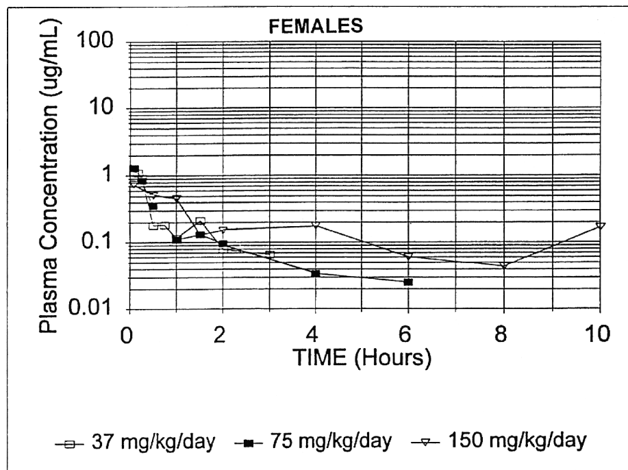
FIGURE I3 Plasma Concentrations of Methyleugenol in Rats at the 18-Month Interim Evaluation in the 2-Year Gavage Study of Methyleugenol
