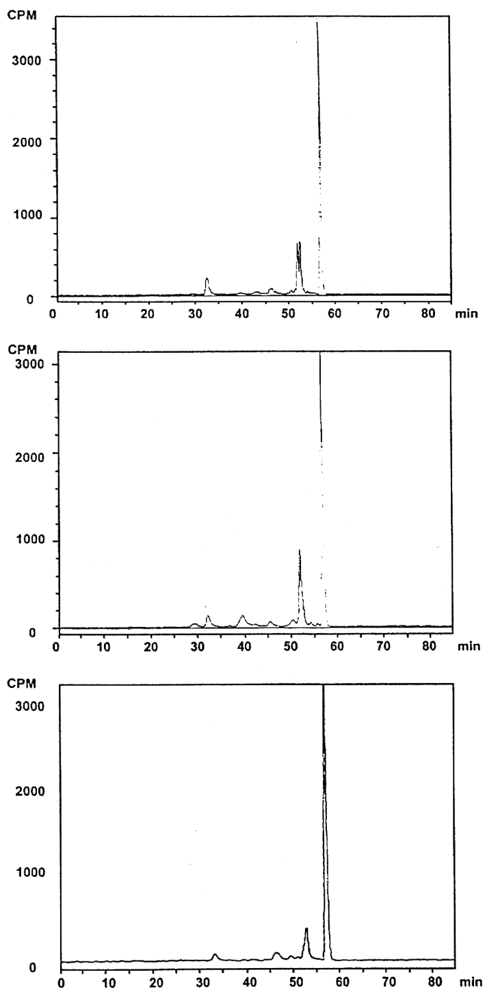
FIGURE N4 Representative Radiochromatograms of Media Taken from Hepatocytes Isolated from Male Fischer 344 Rats, Female B6C3F 1 Mice, and Human Donors Incubated with Methyleugenol for 6 hours. Hepatocytes were incubated with [ 14 C]-methyleugenol for 6 hours at a concentration of 250 μM. Media were harvested, the pH adjusted to 4.0, and analyzed by HPLC. Retention time of methyleugenol is approximately 57 minutes.
