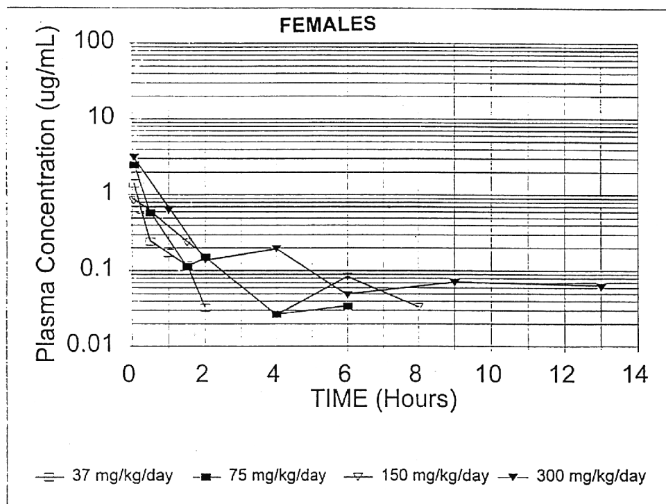
FIGURE II Plasma Concentrations of Methyleugenol in Rats at the 6-Month Interim Evaluation in the 2-Year Gavage Study of Methyleugenol
