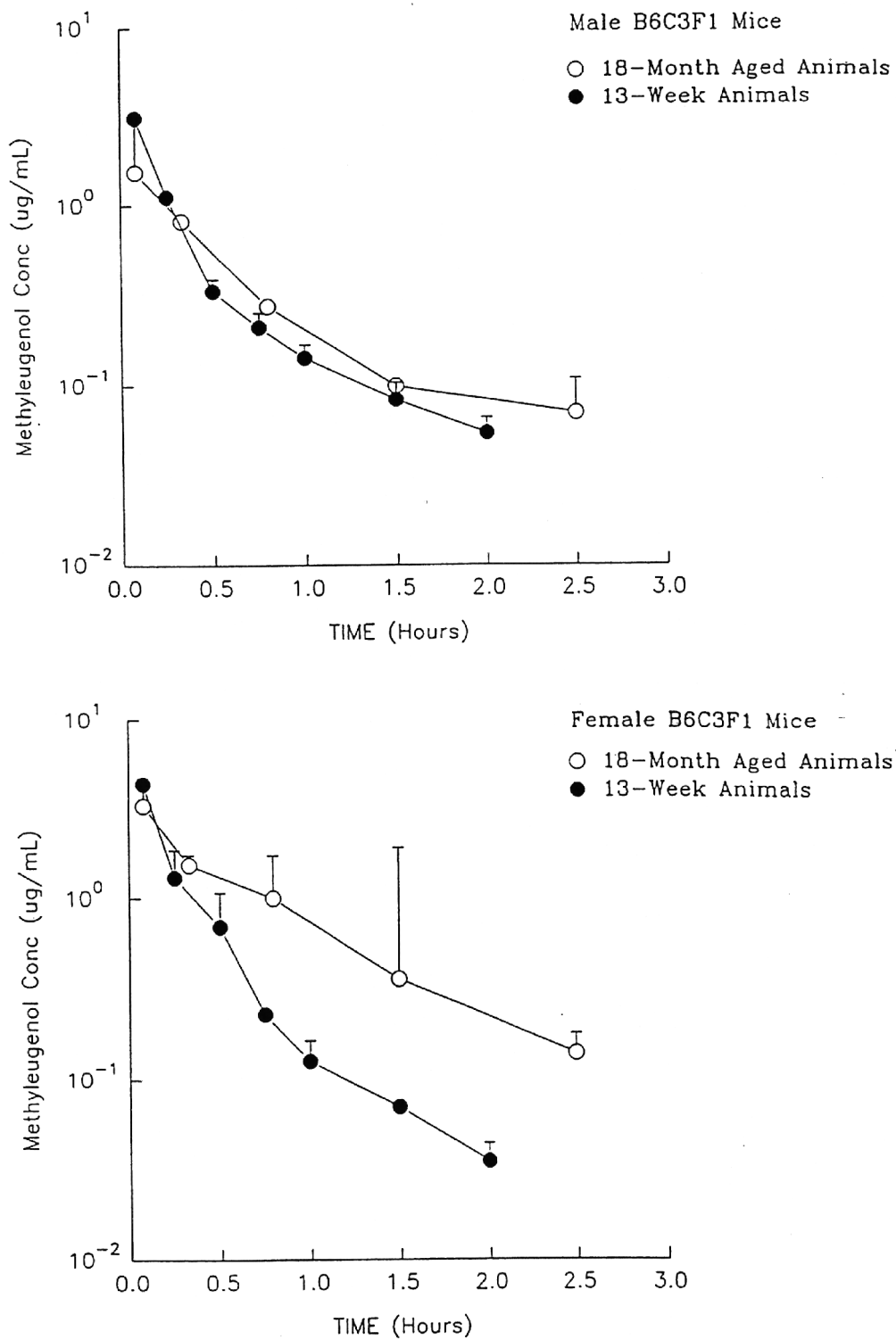
FIGURE II0 Plasma Concentrations of Methyleugenol after a Single Gavage Dose of 75 mg/kg Methyleugenol in Aged and 13-Week-Old Mice
