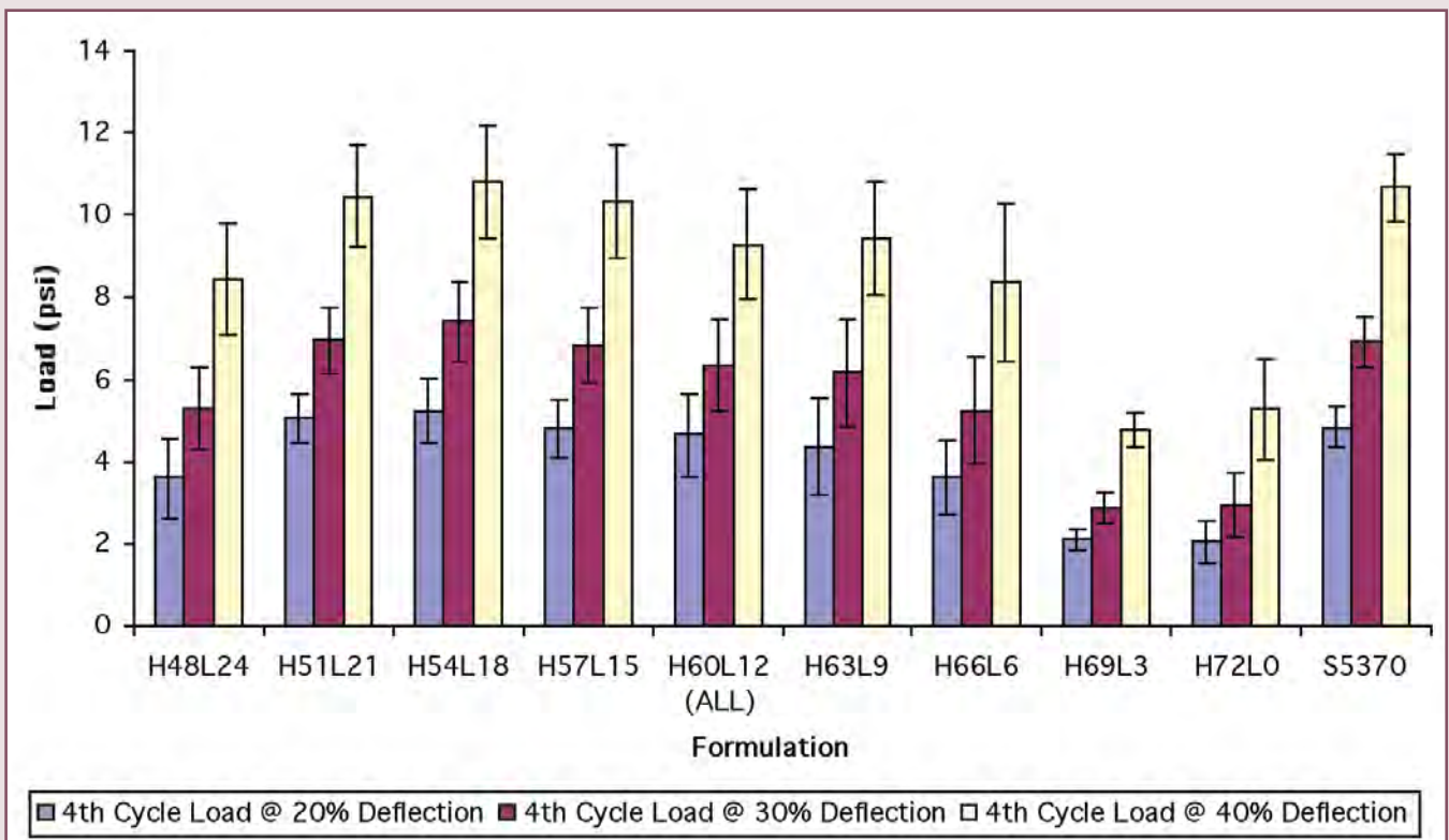
Figure 3. Fourth-cycle load values at 20%, 30%, and 40% deflection for each of the nine LANL formulations and for S5370.
