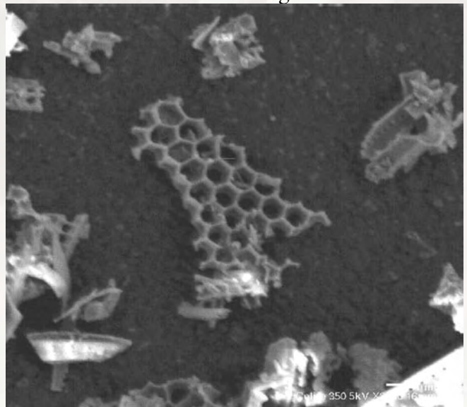
Figure 1. Scanning electron microscope image of diatomaceous earth filler used in S5370 and its replacement, LK3626. Microscopic diatoms are mined from earth deposits. Note the anisotropic shape of some filler particles.
