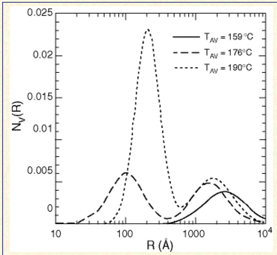
Volume fraction of pores having radius R , measured by SAS techniques, in PBX 9501 that was exposed to a linear thermal gradient. With increasing temperature, a new distribution of pores develops and grows, indicating further microstructural damage.
