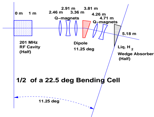
FIG. 40: Schematic diagram of half of a 22.5^\circ bending cell. A wedge absorber is located in the middle of the cell.
