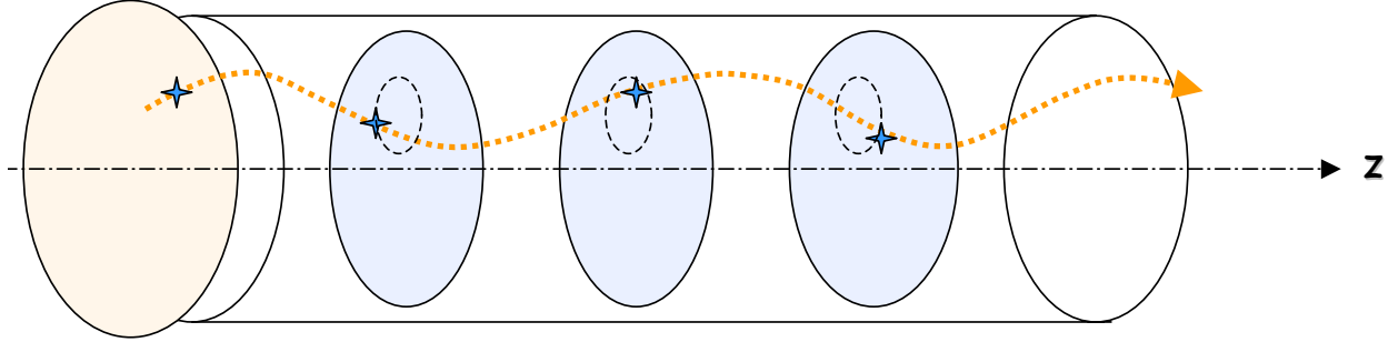
FIG. 46: Conceptual layout of MICE upstream spectrometer: following an initial time-of-flight (TOF) measurement, muons are tracked using detector planes located within a solenoidal magnetic field. Although in principle three x, y measurements as shown suffice to determine the parameters of each muon’s helical trajectory, in practice additional measurement redundancy will be employed; for example, a fourth measurement plane can be used to eliminate very-low-momentum muons that would execute multiple cycles of helical motion. A similar spectrometer (but with the time-of-flight measurement at the end) will be used downstream of the cooling apparatus.
