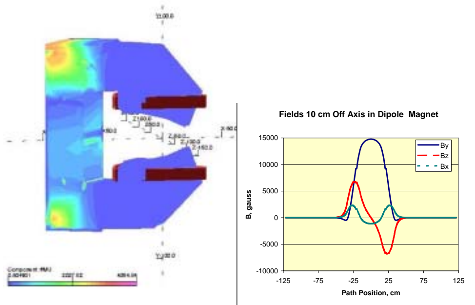
FIG. 36: Figure shows a computer model of a 52cm radius dipole with index n = -\frac{1}{2} and the calculated field components radially 10cm off axis.
