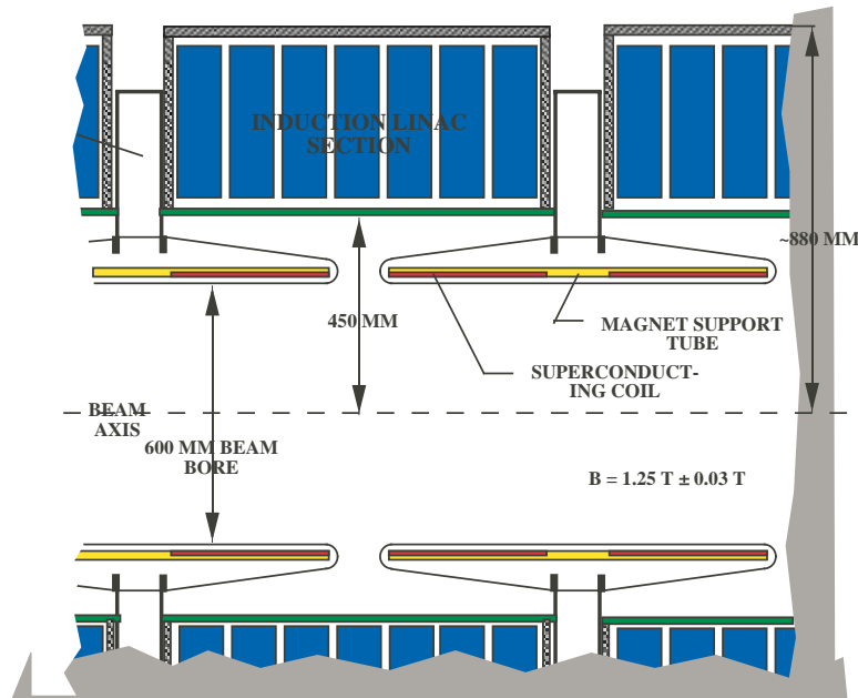
FIG. 15: Cross section of the induction cell and transport solenoids.
