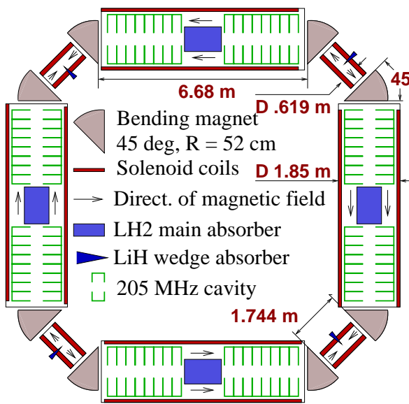
FIG. 34: Layout and parameters of the solenoid based ring cooler
