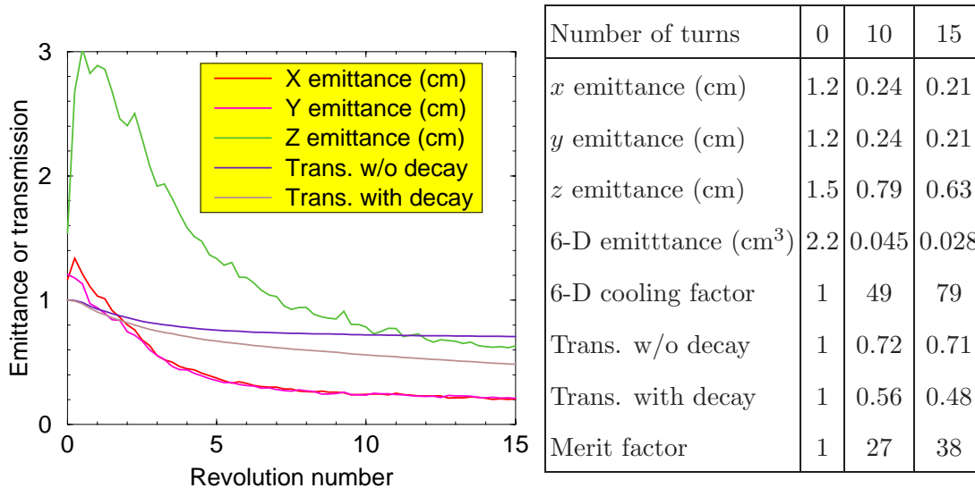
FIG. 35: Evolution of the beam emittance/transmission at the ring cooler.
