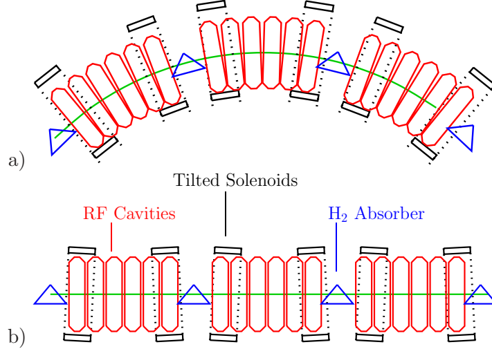
FIG. 38: Three cells of the RFOFO lattice; a) plan, b) side.
