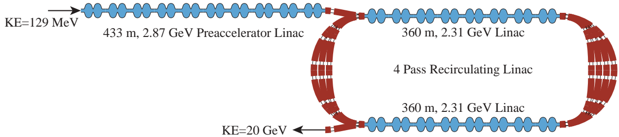
FIG. 21: Accelerating system layout.
