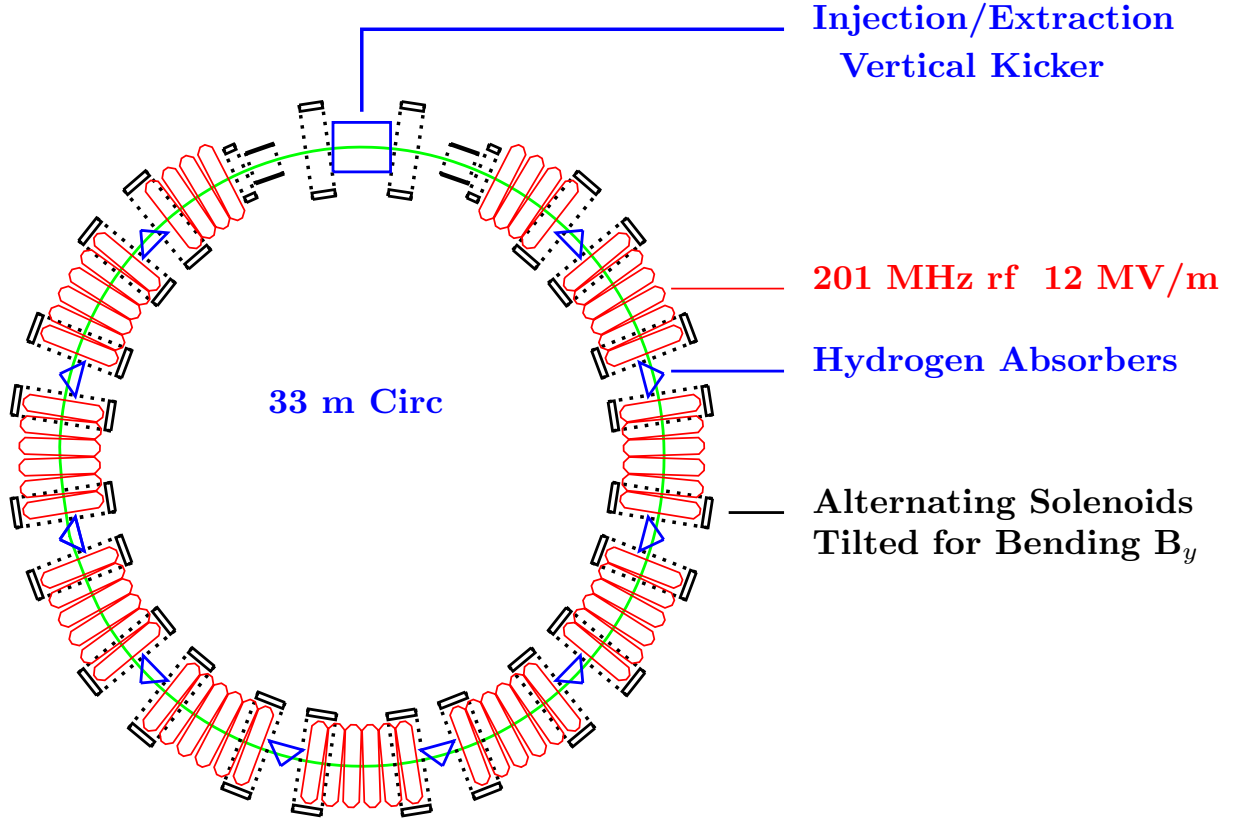
FIG. 37: Layout of an RFOFO cooling ring.
