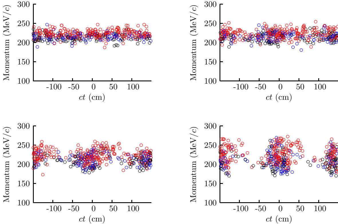
FIG. 17: Evolution of beam in buncher. Plots are at the beginning of the buncher (top left), and at the ends of the three bunching stages (top right, bottom left, and bottom right, in that order).
