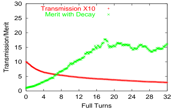
FIG. 44: The transmission and the figure of merit factor as a function of the arc length in 32 full turns.
