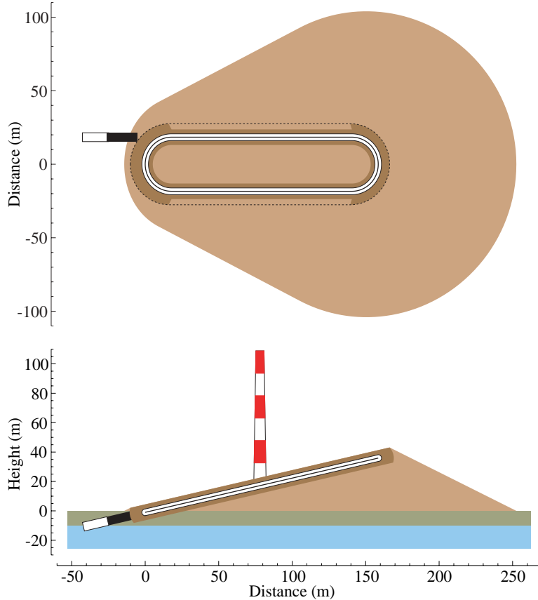
FIG. 26: Top view and cross section through 20 GeV ring and berm. The existing 110 m tower, drawn to scale, gives a sense of the height of the ring on the BNL landscape.
