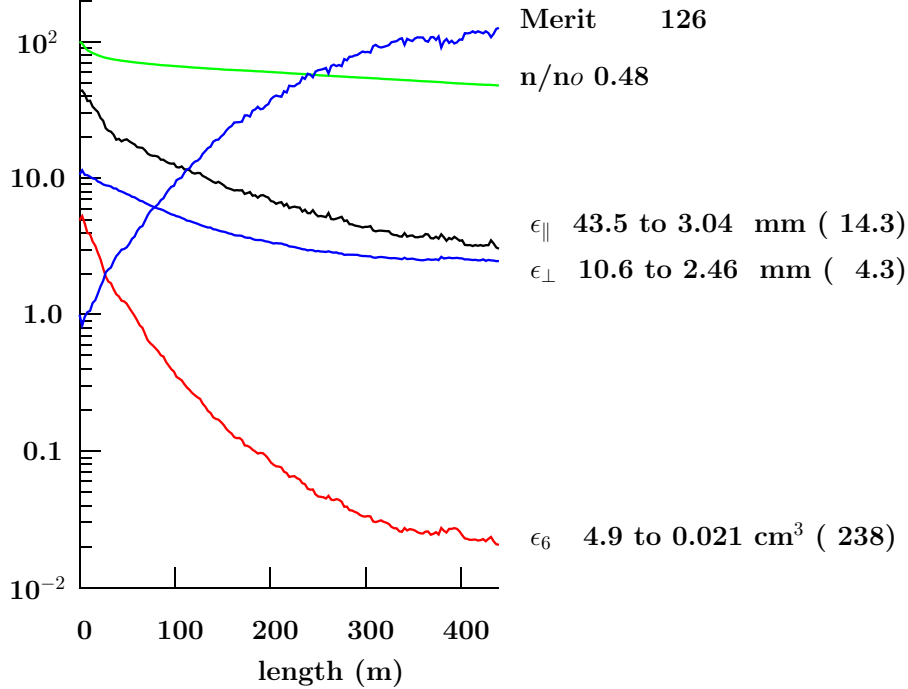
FIG. 39: Transmission, normalized transverse emittance, normalized longitudinal emittance, normalized 6-dimensional emittance, and the merit factor, as a function of distance.
