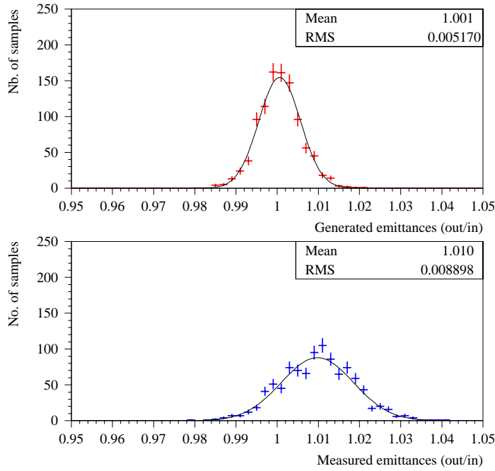
FIG. 49: Distribution of ratios of output to input six-dimensional emittance for 1000 simulated experiments, each with 1000 accepted muons. The top figure shows the distribution of this ratio for the emittances as generated by simulation; the bottom figure, as “measured” in the simulated experiments. The curves are Gaussian fits to the points.
