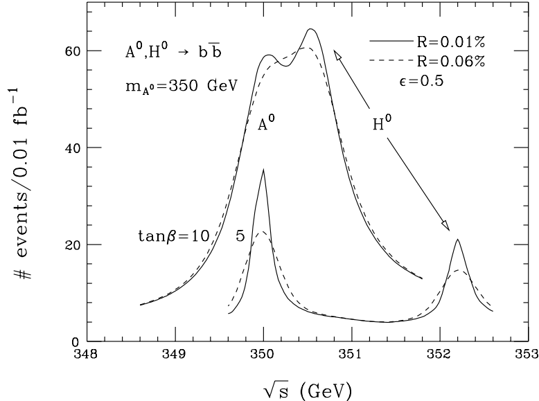
FIG. 11: Separation of A and H signals for \tan\beta = 5 and 10 . From Ref. [117].
