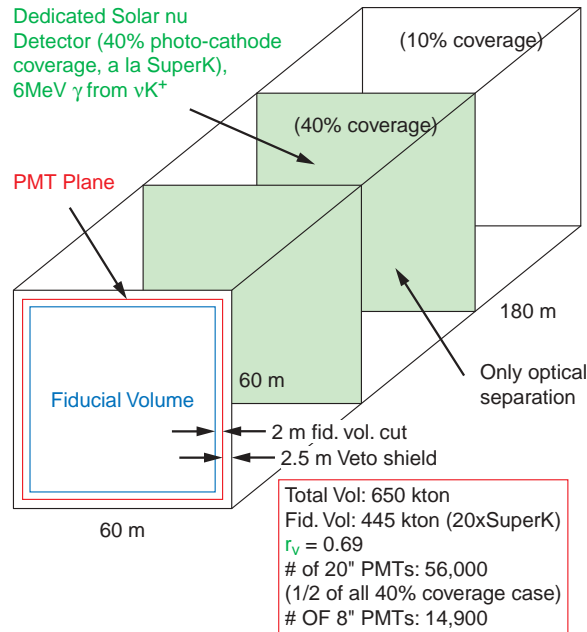
FIG. 29: A possible 50 kton steel-scintillator-PDT detector at WIPP.
