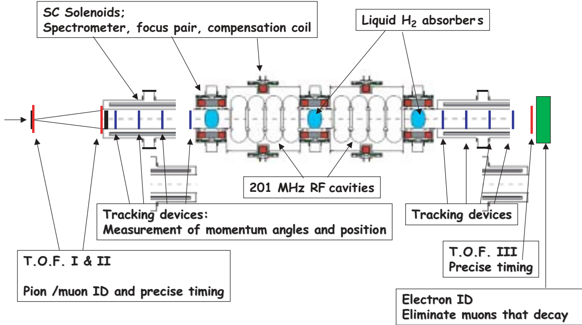
FIG. 47: Schematic layout of MICE apparatus.
