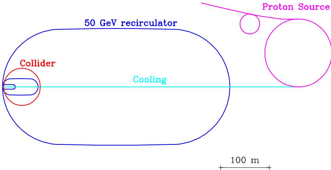
FIG. 33: Plan of a 0.1-TeV-CoM muon collider, also known as a Higgs Factory.
