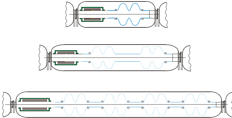
FIG. 22: Layouts of short (top), intermediate (middle) and long (bottom) cryomodules. Blue lines are the SC walls of the cavities. Solenoid coils are indicated in red.
