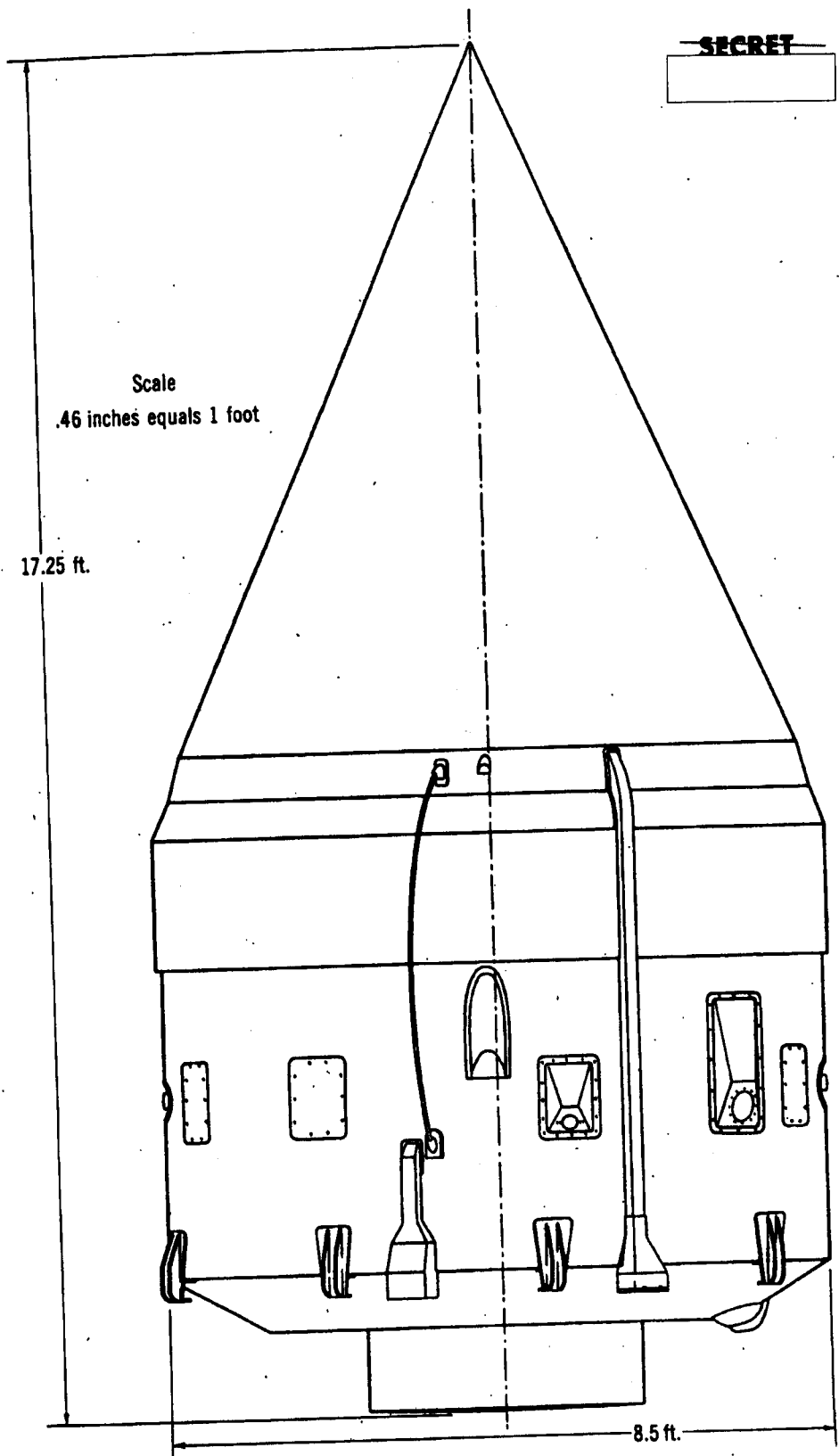
Figure 8. Lunik 1 last stage vehicle, side 2
