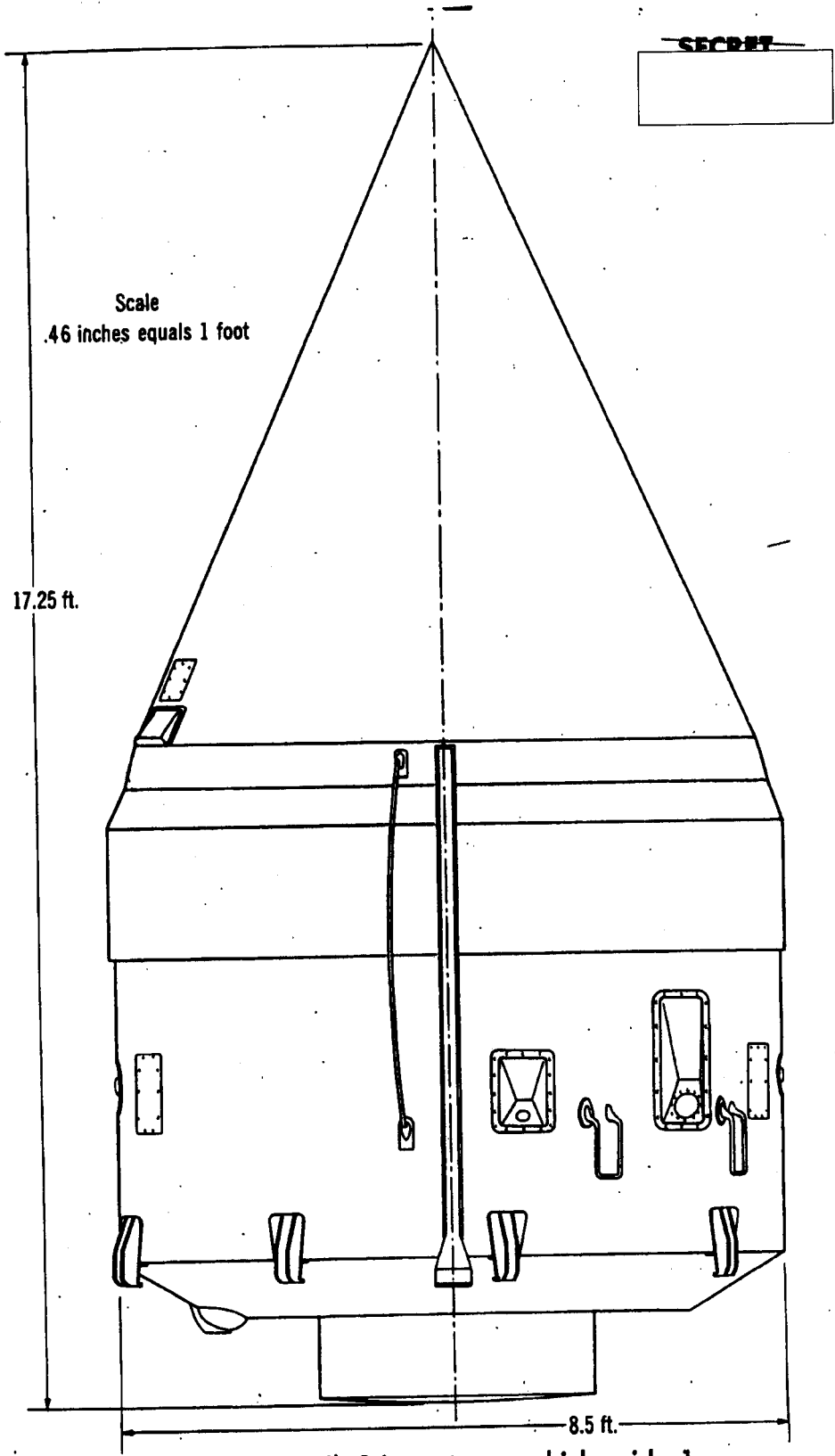
Figure 7. Lunik 1 last stage vehicle, side 1
