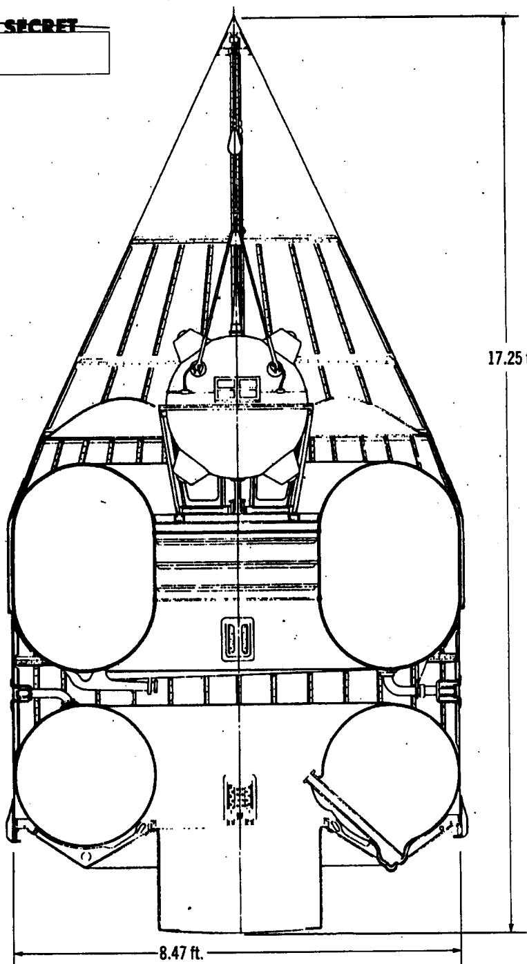
Figure 6. Diagram of Lunik-1 last stage vehicle
