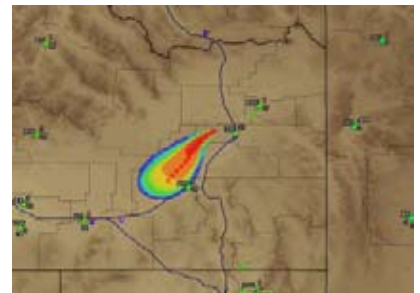
Example of a HYSPLIT model concentration isopleth map displayed using an ARL Rapid Response Tool for a theoretical release scenario in Southeastern Idaho.
