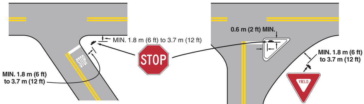
ACUTE ANGLE INTERSECTION
