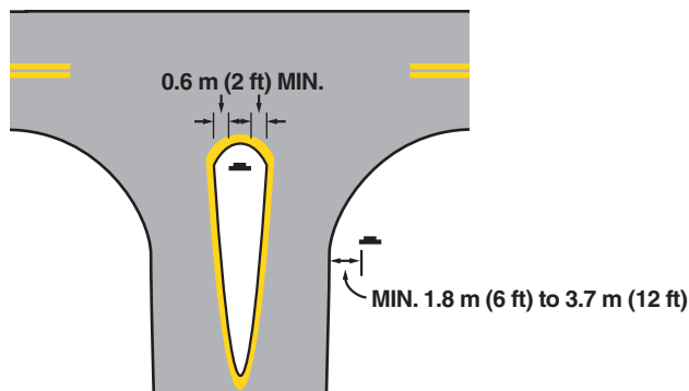
DIVISIONAL ISLAND
