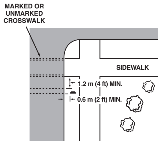
URBAN INTERSECTION
