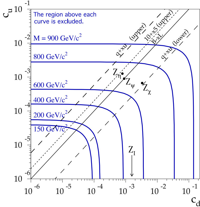
Figure 2: Exclusion region in the c_u - c_d plane (see Eq. (7)) for given M_{Z'} . Figure adapted from [14].
