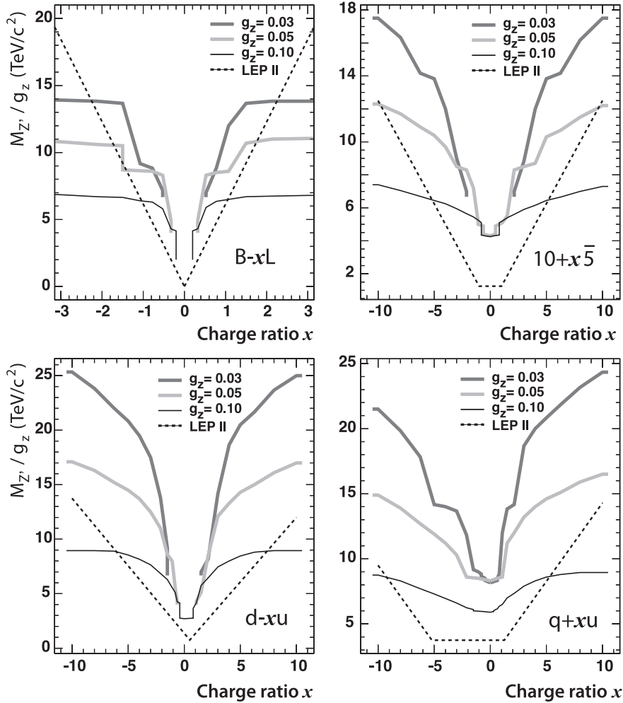
Figure 1: Exclusion limits on the sets of U(1) charges shown in Table 1, from CDF (for different values of the gauge coupling g_z ) and the LEP-II experiments (adapted from [13]). The CDF analysis combined the invariant mass and angular distributions of the e^+e^- final state.
