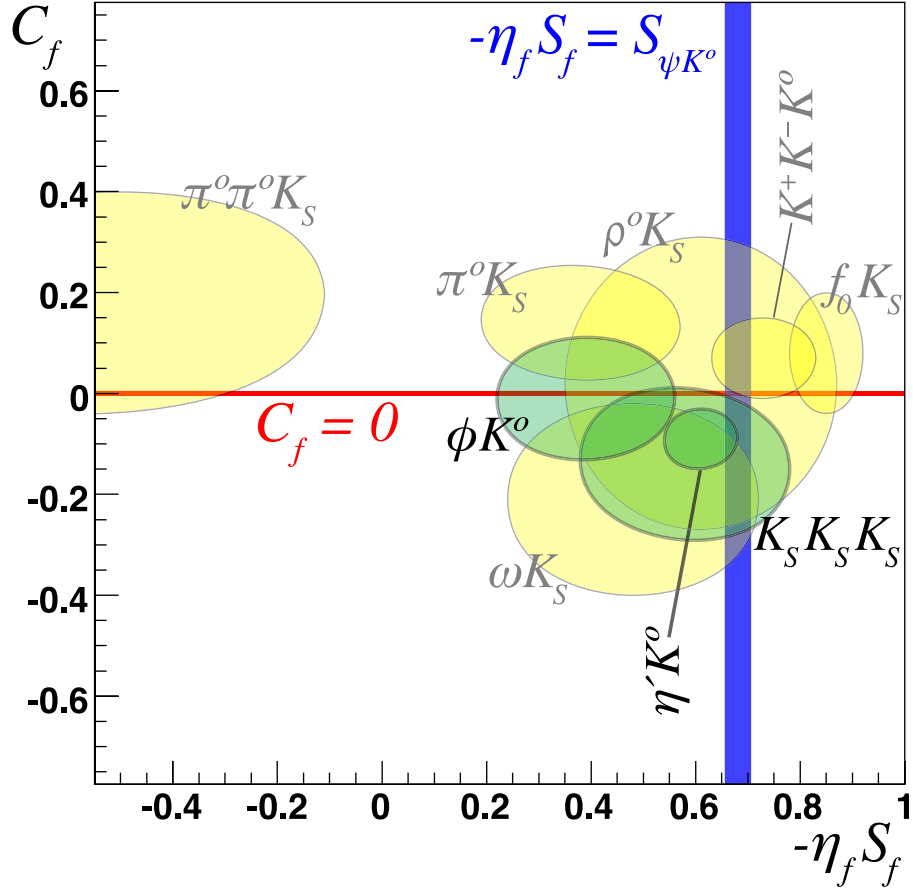
Figure 12.3: Summary of the results [20] of time-dependent analyses of b \rightarrow q\bar{q}s decays, which are potentially sensitive to new physics. Subdominant corrections are expected to be smallest for the modes shown in green (darker). Results for final states including K^0 mesons combine CP -conjugate K_S and K_L measurements. The final state K^+K^-K^0 is not a CP eigenstate; the mixture of CP -even and CP -odd components is taken into account in obtaining an effective value for \eta_f S_f . Correlations between C_f and S_f are included when available.
