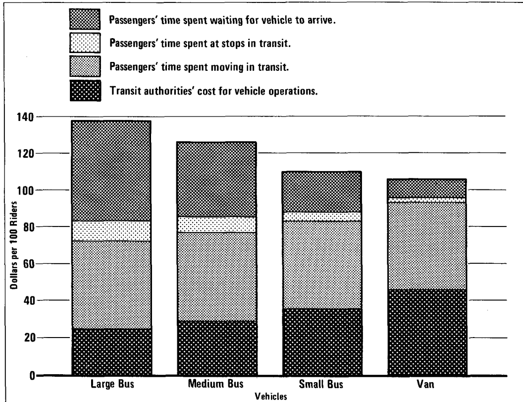
Figure 3. Comparison of 1984 Public Transit Costs for Four Vehicle Types (Costs in 1984 dollars)
