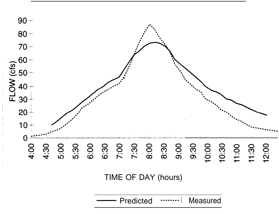
Exhibit 7-11. Flow Hydrograph
