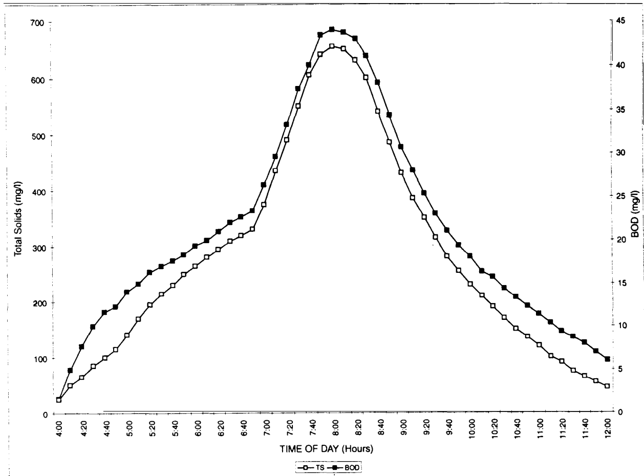
Exhibit 7-12. Pollutographs
