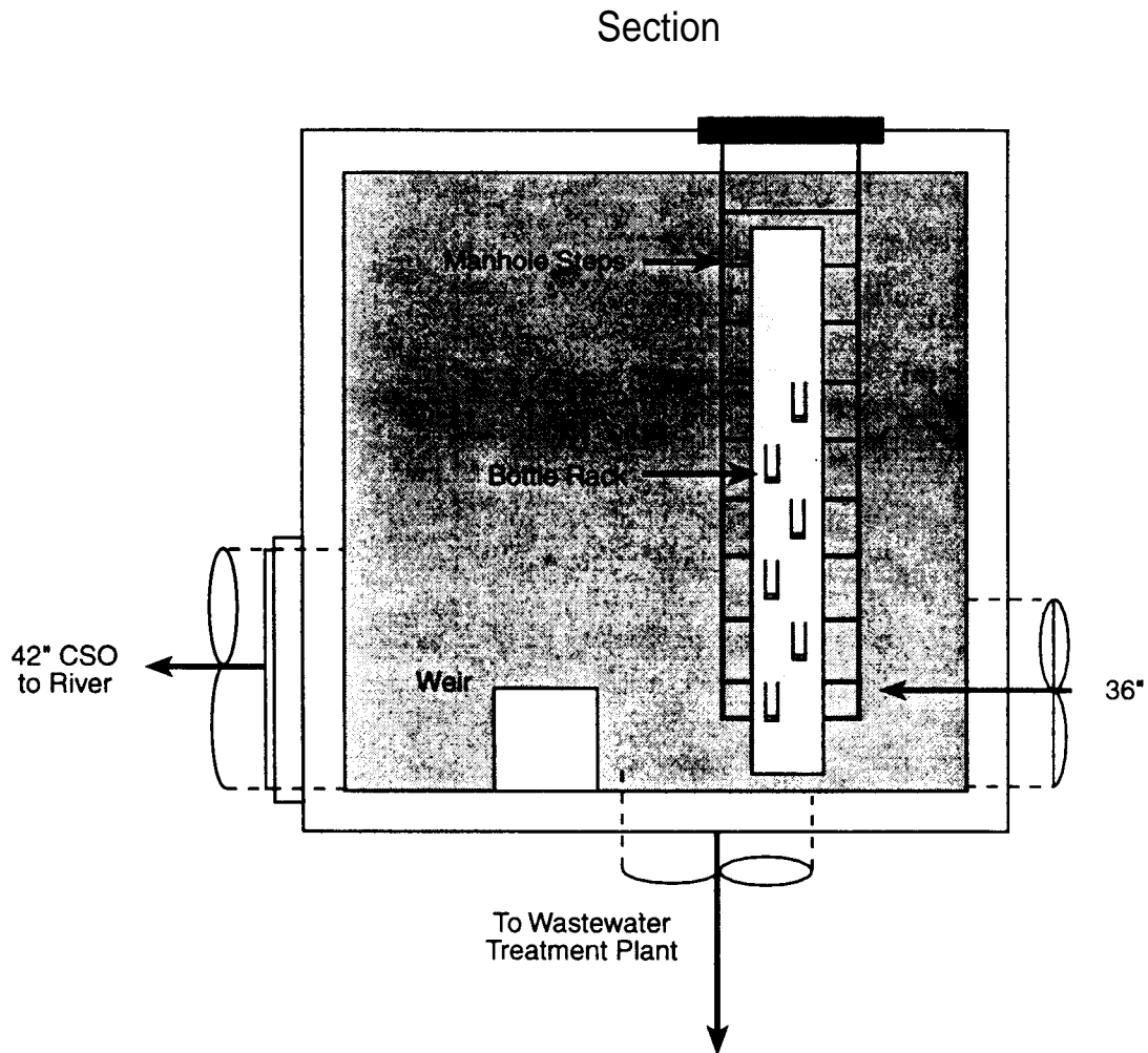
Exhibit 5-6. Illustration of a Bottle Board Installation
