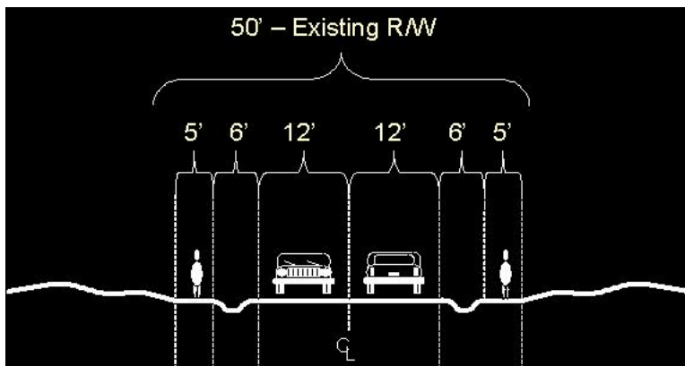
Figure 36: Rural section
