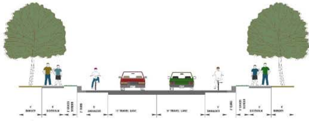
TYPICAL MULTIMODAL SERVICE ROAD CROSS-SECTION (SEE REQUIRED RIGHT-OF-WAY)
