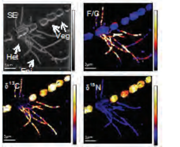
Figure. NanoSIMS images of a chain of 8 cells from the filamentous cyanobacterium Anabaena sp. SSM-00 with cells of the \alpha -Proteobacterium epibiont Rhizobium sp. WH2K attached to a heterocyst. Images were taken after 24 h of incubation with \text{H}^{13}\text{CO}_3^- and ^{15}\text{N}_2 . SE: Secondary electron image showing the location of all cells. F/C: Fluorine is enriched in the epibiont relative to Anabaena after in situ hybridization with an \alpha -Proteobacteria specific probe (scale, 0 – 0.2). \delta^{13}\text{C} : ^{13}\text{C} enrichment image showing the relative uptake of newly fixed carbon (scale, 0 – 300 parts per thousand). \delta^{15}\text{N} : ^{15}\text{N} enrichment image showing the relative uptake of newly fixed nitrogen (scale 0 – 15,000 parts per thousand). The color bars indicate the relative enrichment of the isotope in the image. Het, heterocyst; Veg, vegetative cells; Epi, epibiont.
