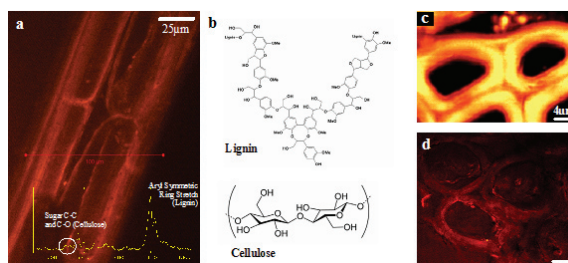
Figure. a) CARS images of cross section of corn stover cell walls by integrating over the aromatic lignin band wavelength ( 1,550\text{--}1,640\text{ cm}^{-1} ). b) Chemical Structures of lignin and cellulose. c) Cross section of poplar wood imaged by Raman microscopy (integration time of 55 min) and d) CARS microscopy (integration time of 20sec).
