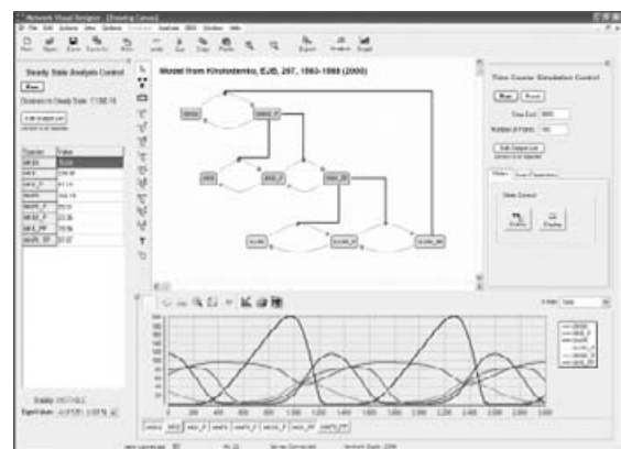
Sauro - Fig. 1. JDesigner simulating a MAPK Pathway
