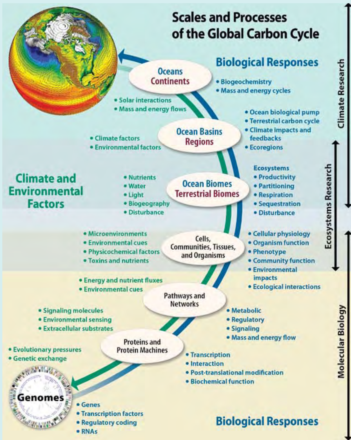
Fig. 2.1. Scales and Processes of the Global Carbon Cycle. The global carbon cycle is determined by the interactions of climate, the environment, and Earth’s living systems at many levels, from global to molecular. Relating processes, phenomena, and properties across spatial and temporal scales is critical for deriving a predictive mechanistic understanding of the global carbon cycle to support more precise projections of climate change and its impacts. The domains of climate, ecosystem, and molecular biology research each has a limited reach in scales, constrained by the complexity of these systems and limitations in empirical and modeling capabilities. While linking comprehensively from genomes to global phenomena is intractable, many connections at intermediate scales are viable with integrated application of new systems biology approaches and powerful analytical and modeling techniques at the physiological and ecosystem levels. Biological responses (blue) are to the right of the systems ovals, and climate and environmental factors (green) are to the left of the systems ovals. [Note: Globe portion of figure courtesy of Gary Strand, National Center for Atmospheric Research, with funding from the National Science Foundation and the Department of Energy.]
