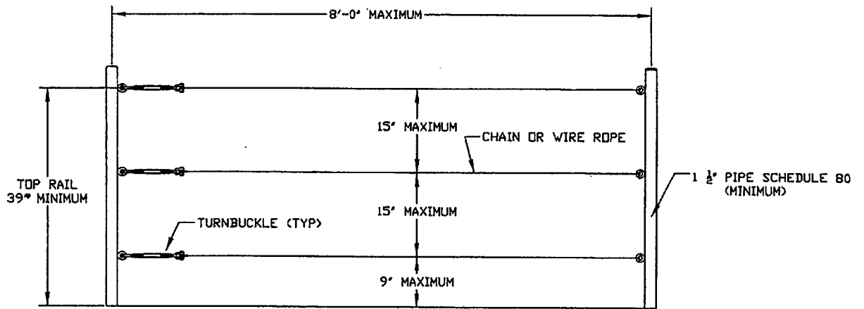
MARINE TYPE B THREE TIER TENSIONED RAILING
