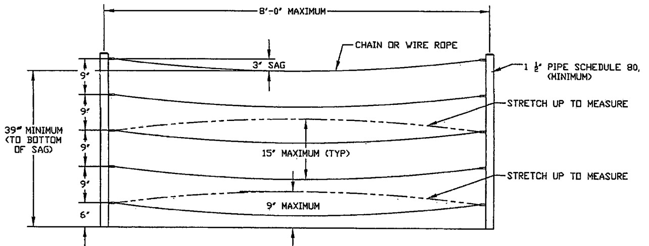
MARINE TYPE C NON-TENSIONED RAILING (3" SAG SHOWN)
