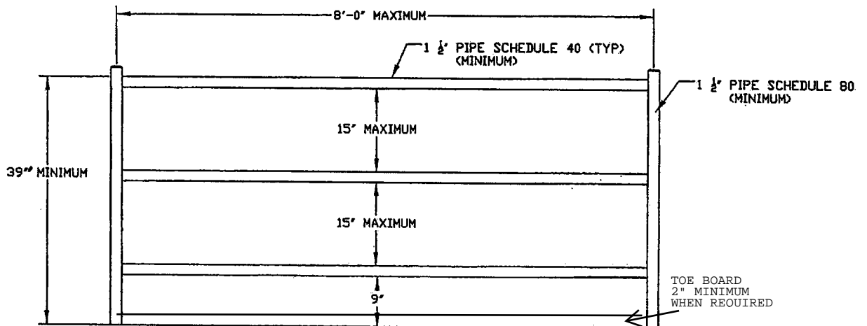
MARINE TYPE B THREE TIER RIGID RAILING
