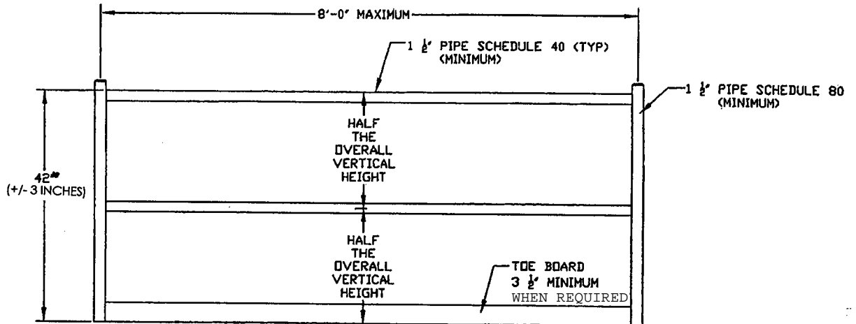
MARINE RAILING TYPE A, TWO TIER RIGID FALL PROTECTION RAILING
