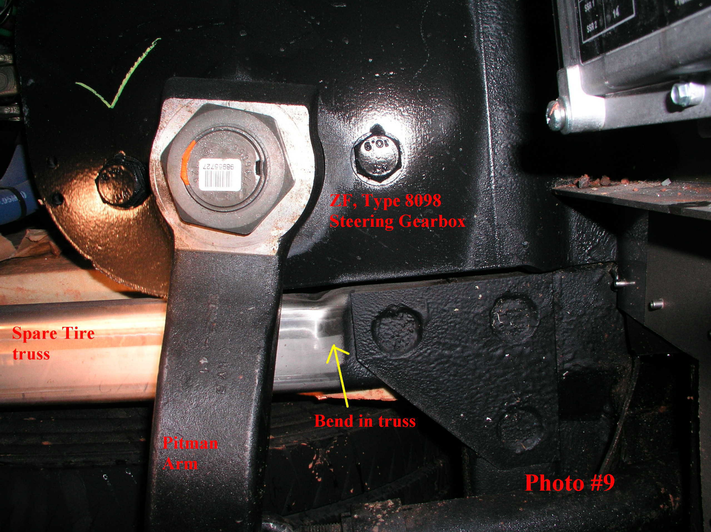
Veh. Photo #09 - Crease in spare tire truss near the firewall
