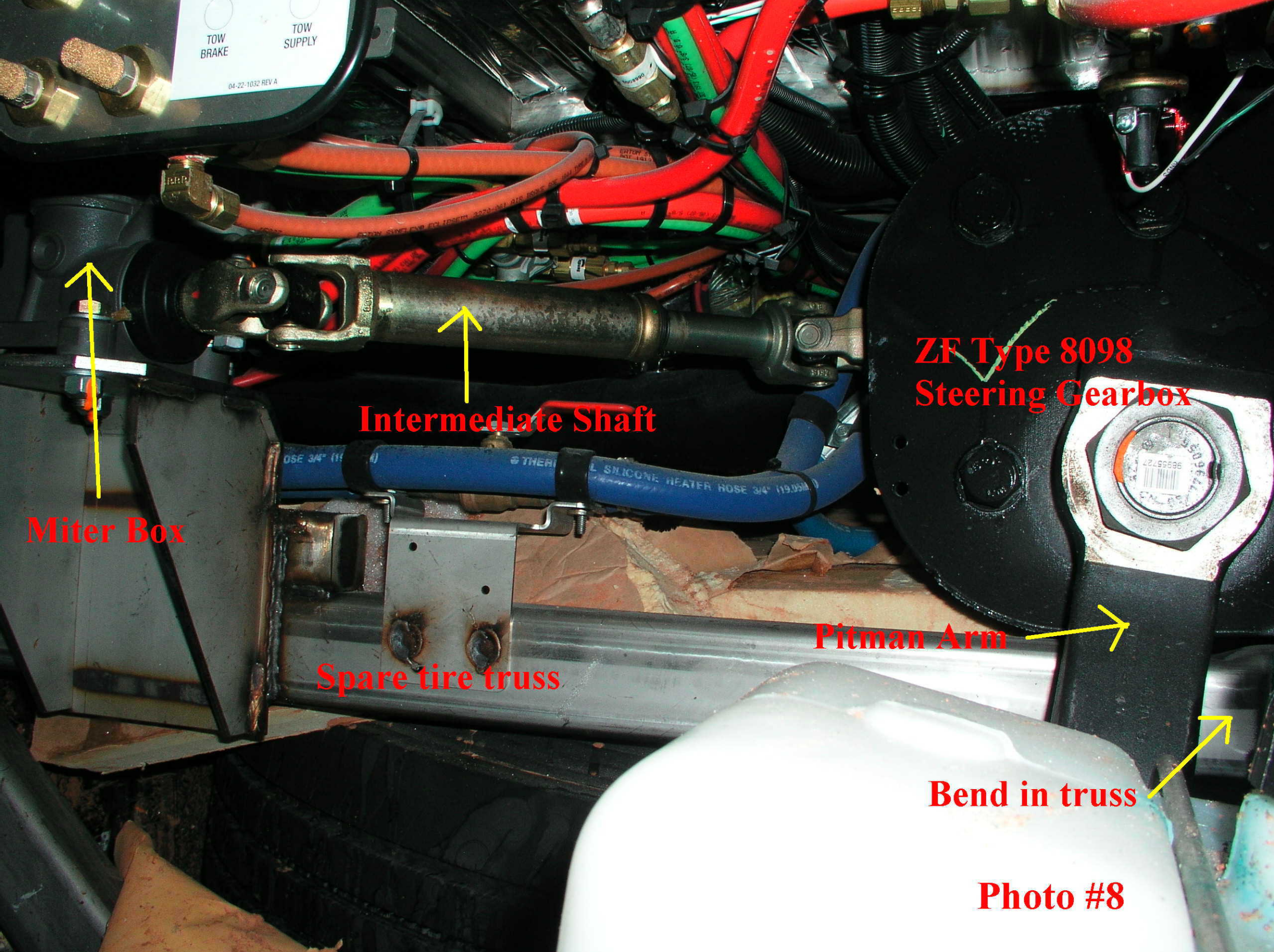
Veh. Photo #08 - Photo with miter box on the left with intermediate shaft attached. The spare tire truss, upon which the miter box is mounted is bowed up, as evidenced by the crease in the truss that can be seen at the very right edge of the photo,
