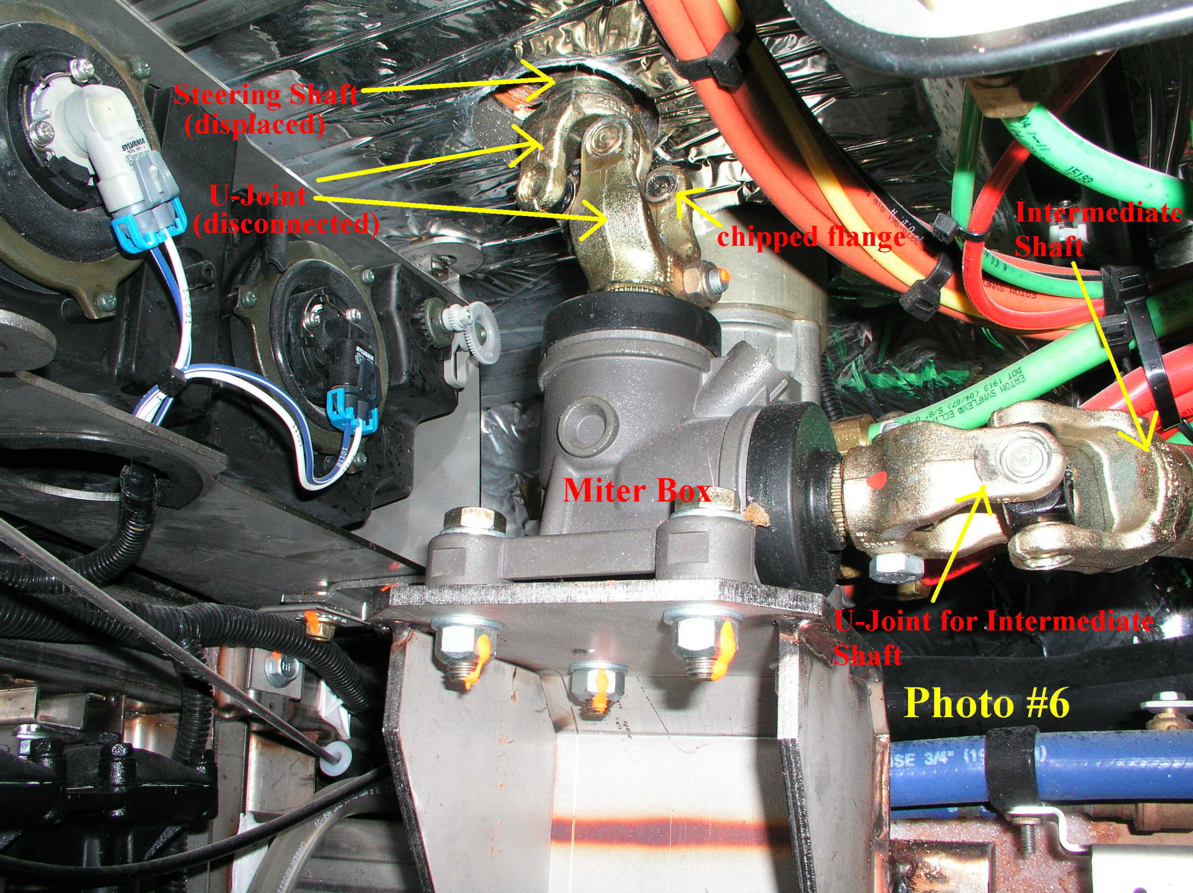
Veh. Photo #6 - Miter box with steering shaft (top center of photo) separated at the input shaft U-joint
