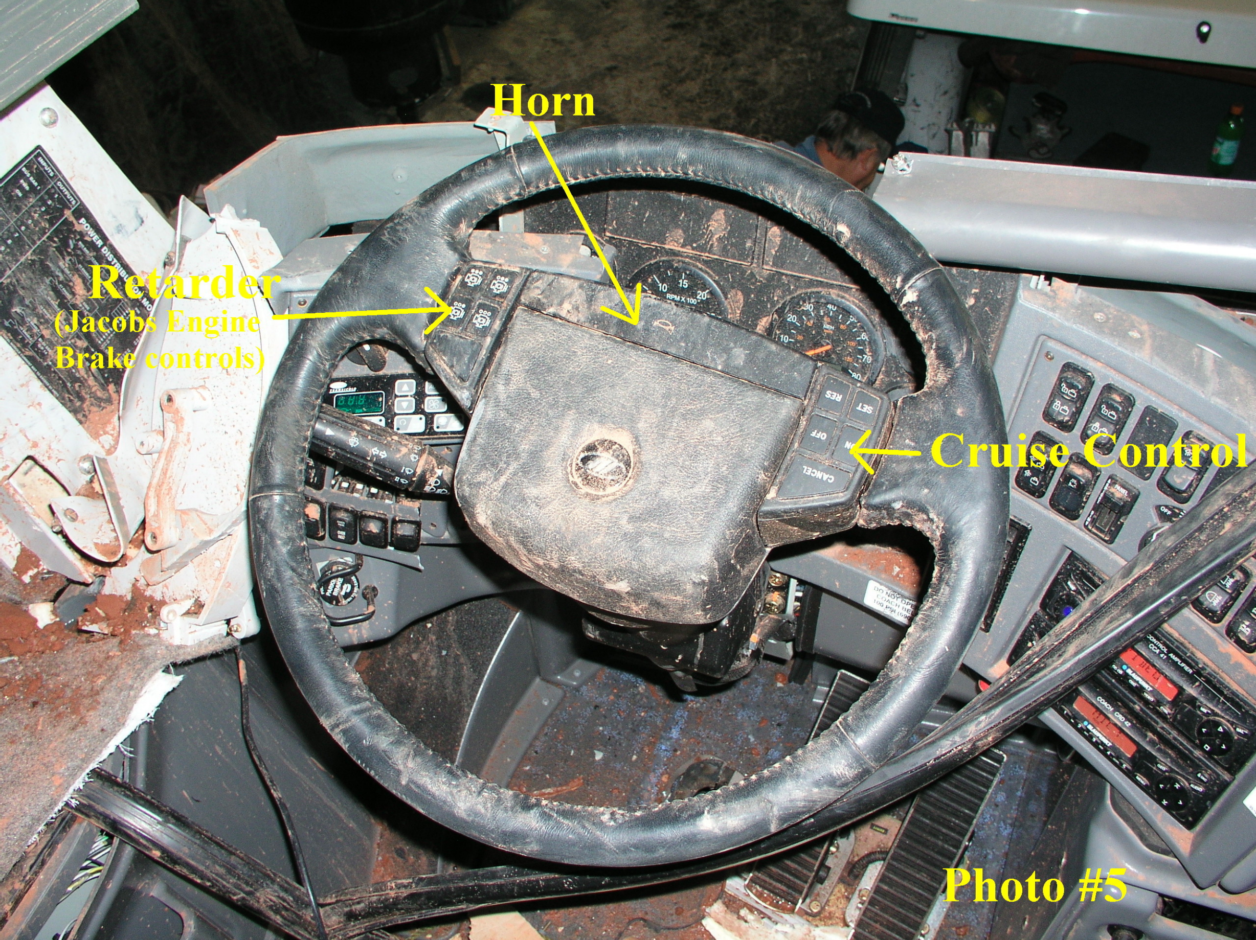
Veh. Photo #05 - SmartWheel steering wheel (Note: Steering wheel is turned in an inverted position, with the cruise control switches on the right and engine brake on the
