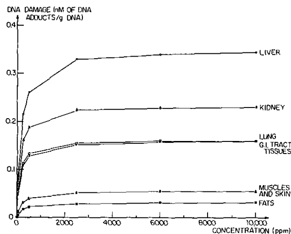
FIGURE 32. Effective dose to the liver (DNA adducts, in nM/g DNA) versus vinyl chloride exposure, predicted by a pharmacokinetic compartment model (57).
