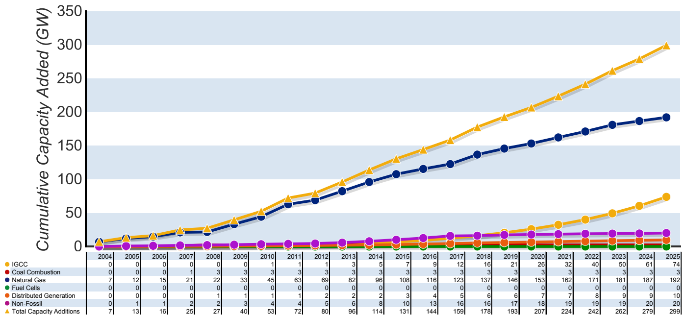
Figure 6-2: Cumulative Additions of Electricity Generation Capacity, 2004–2025 Under Multi-Pollutant Regulation
