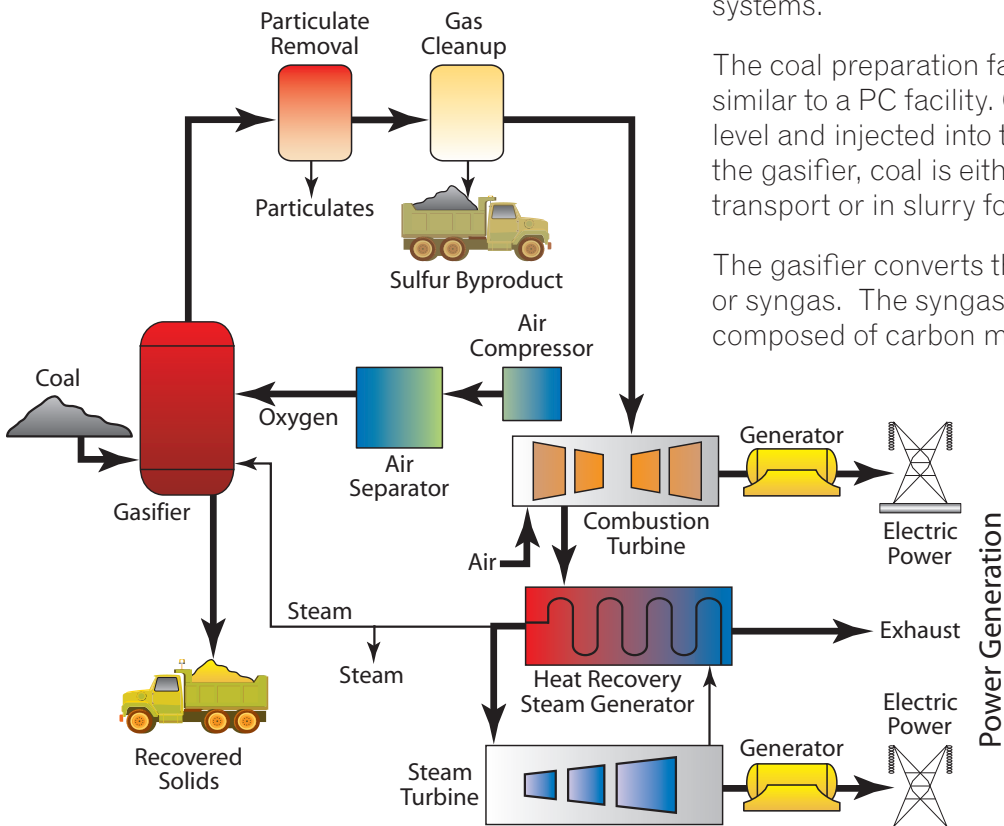
Figure 1-1: Coal-based IGCC
