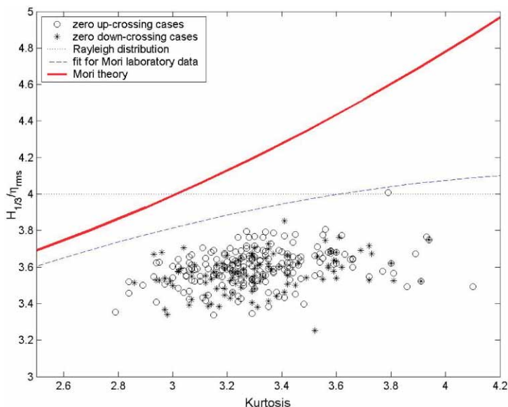
Figure 12. Relationship between kurtosis and normalized H_{1/3} ( H_{1/3}/\eta_{\text{rms}} ).
