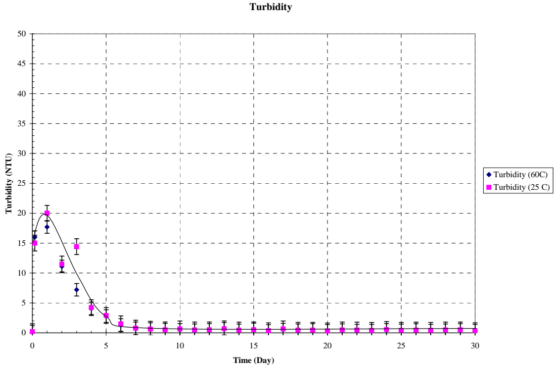
Figure 4-70. Turbidity results.
