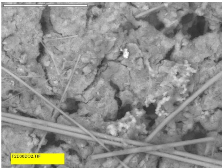
Figure 4-64. Higher-magnification ESEM image of a Test #2, Day-30 exterior fiberglass sample on the drain collar (away from the drain screen). The image shows particulate deposits on the fiberglass.
