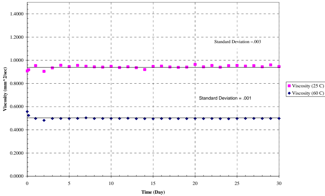
Figure 4-72. Viscosity at 60°C and 25°C.
