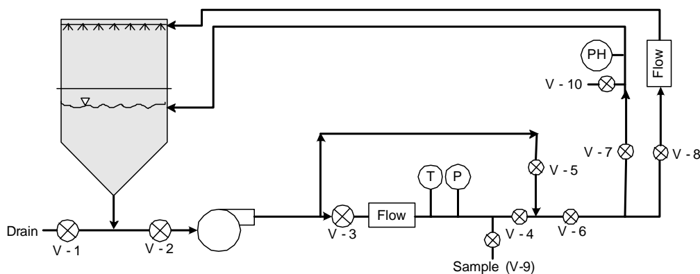
Figure 3-1. Test loop process flow diagram.
