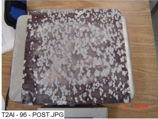
Figure 4-3. A1-96 submerged, post-test.
