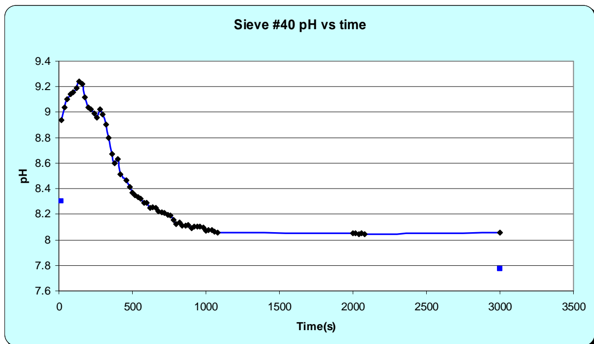
Figure 2: Effluent pH with a 1-inch layer of # 40 slag, a flow rate of 800mL/min, and tap water.
