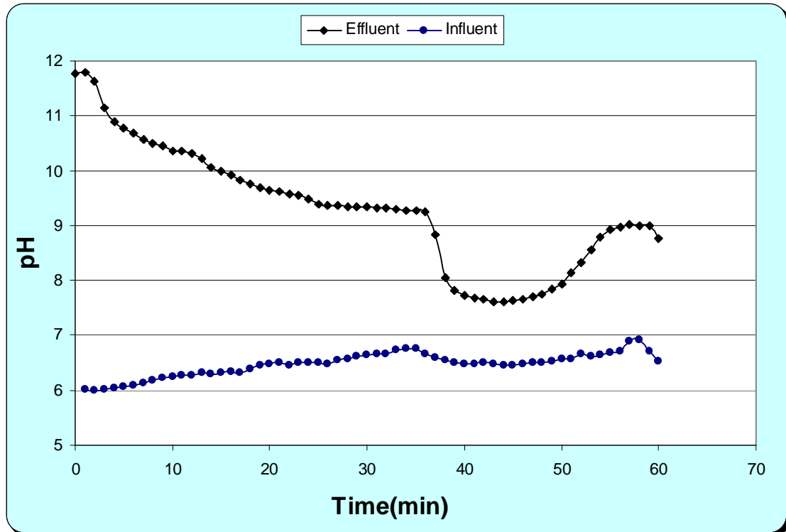
Figure 3: Influent and effluent pH with slag #60, a bed depth of 2 in, a flow rate of 800 mL/min, and acidic influent.
