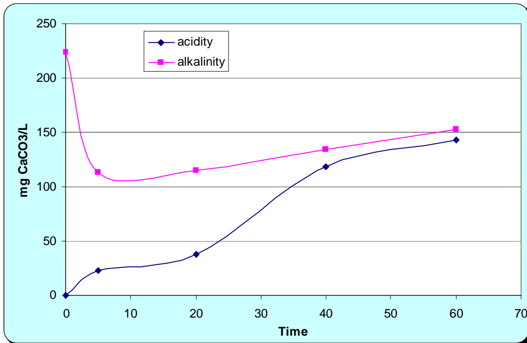
Figure 4: Effluent alkalinity and acidity plotted against the time with slag #60, a bed depth of 2 in, a flow rate of 800 mL/min, and an acidic influent.
