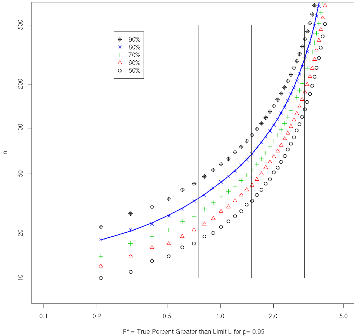
Sample Sizes For H_0: F_p < 5\text{Percent} Equivalent To H_0: X_p > L_p p=0.95 For Power = 50% to 90% Vertical Lines at F^* = 0.75\% 1.5% and 3%
